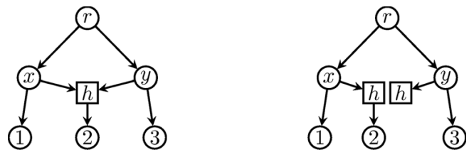
Figure 2 Computing the eNewick string of a phylogenetic network. A phylogenetic network N (left), and tree (right) associated to N for computing its eNewick string.
