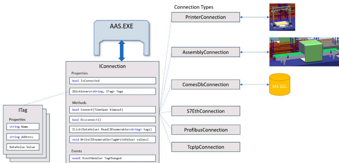
Figure 11. Integration of different communication drivers without rebuilding the AAS.
