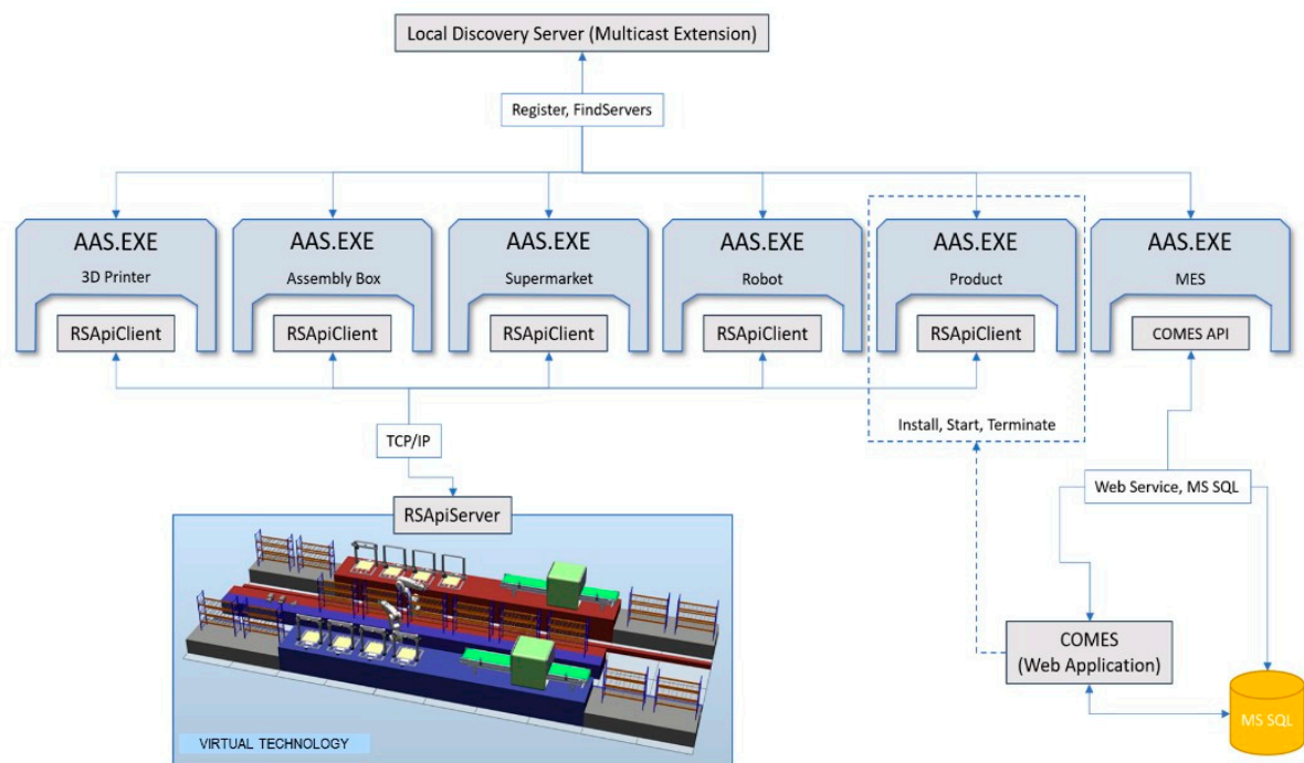
Figure 6. The architecture of the presented case study.
