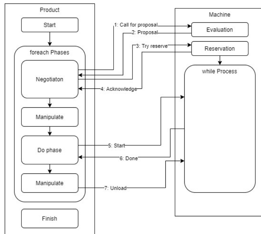
Figure 12. The architecture and flow of the discrete event simulation scenario.
