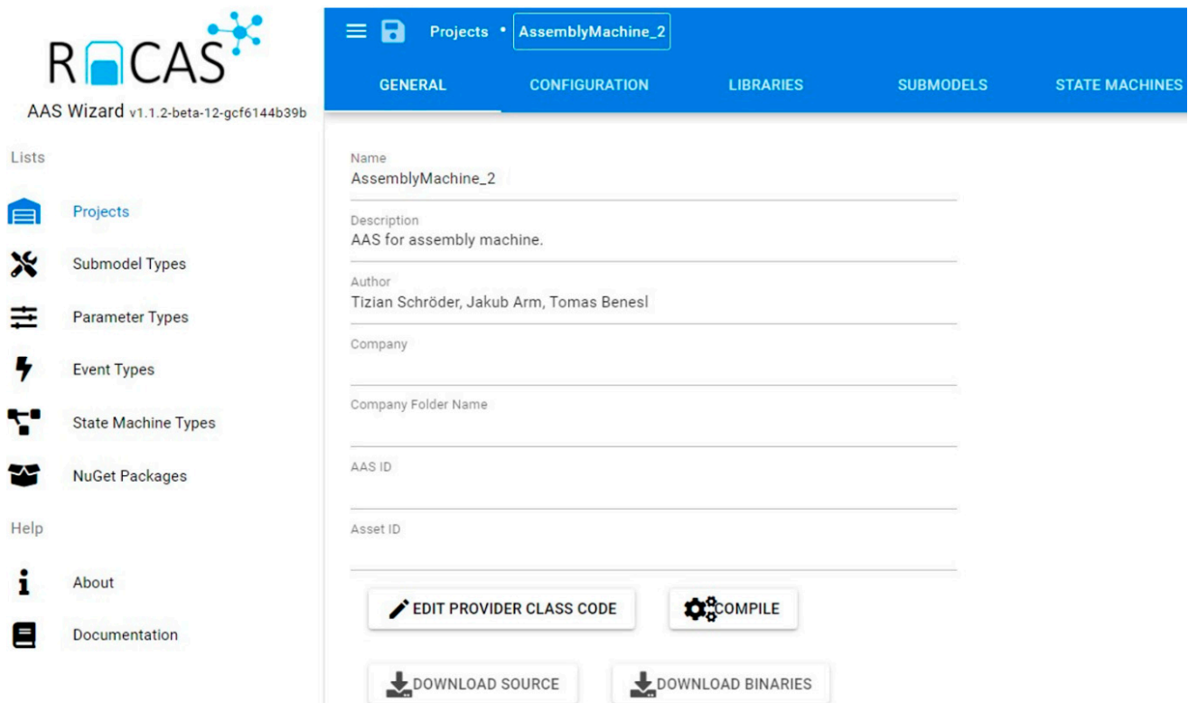
Figure 5. A ConfigWizard screenshot: front end.
