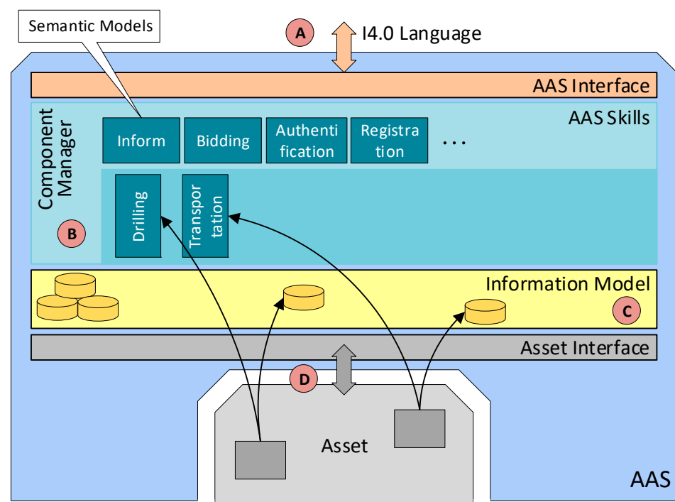
Figure 10. A block diagram of an AAS.
