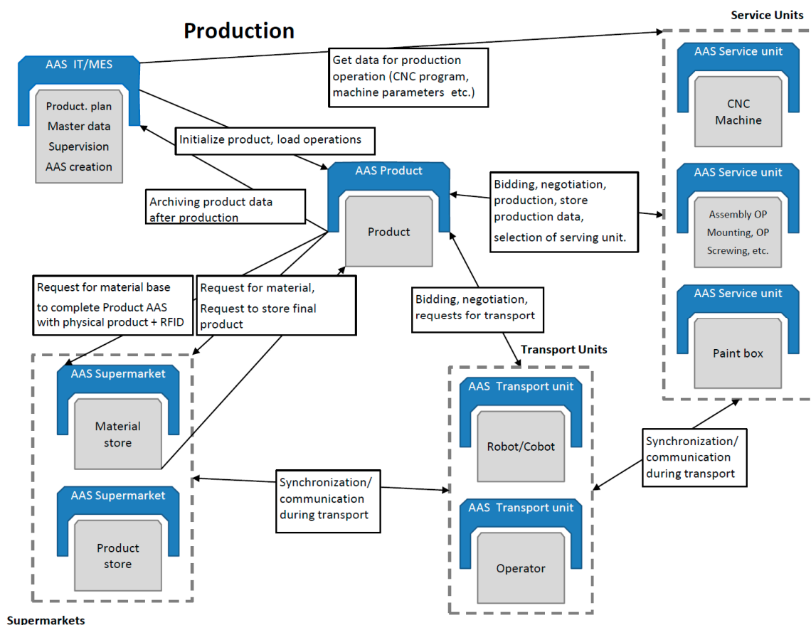
Figure 8. The data flow in a smart factory.
