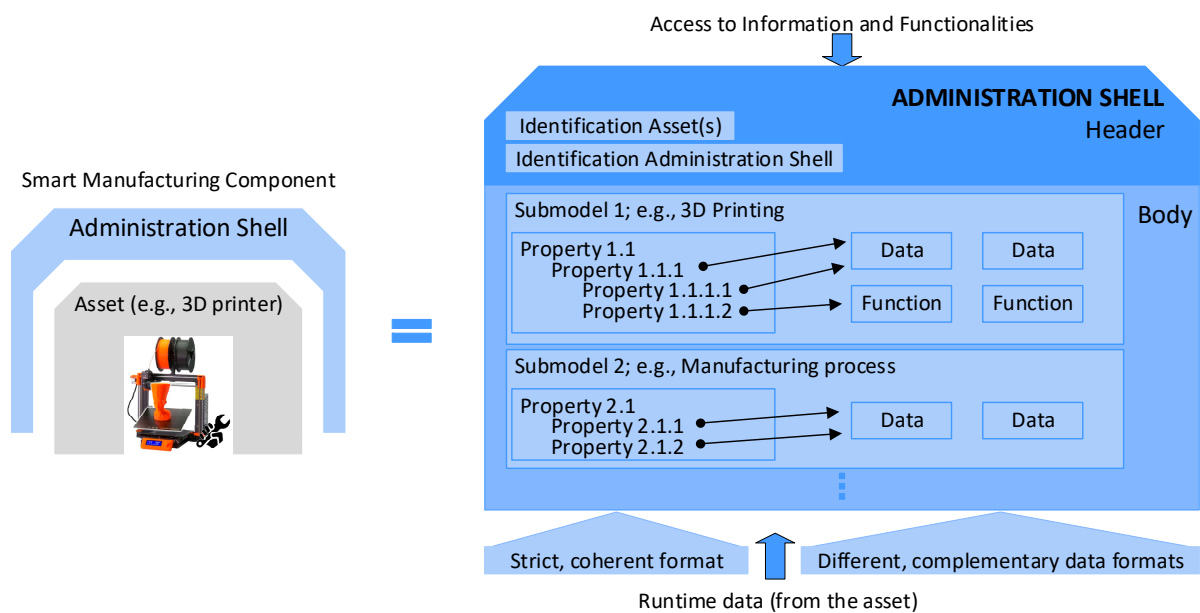
Figure 1. The detailed structure of an AAS.
