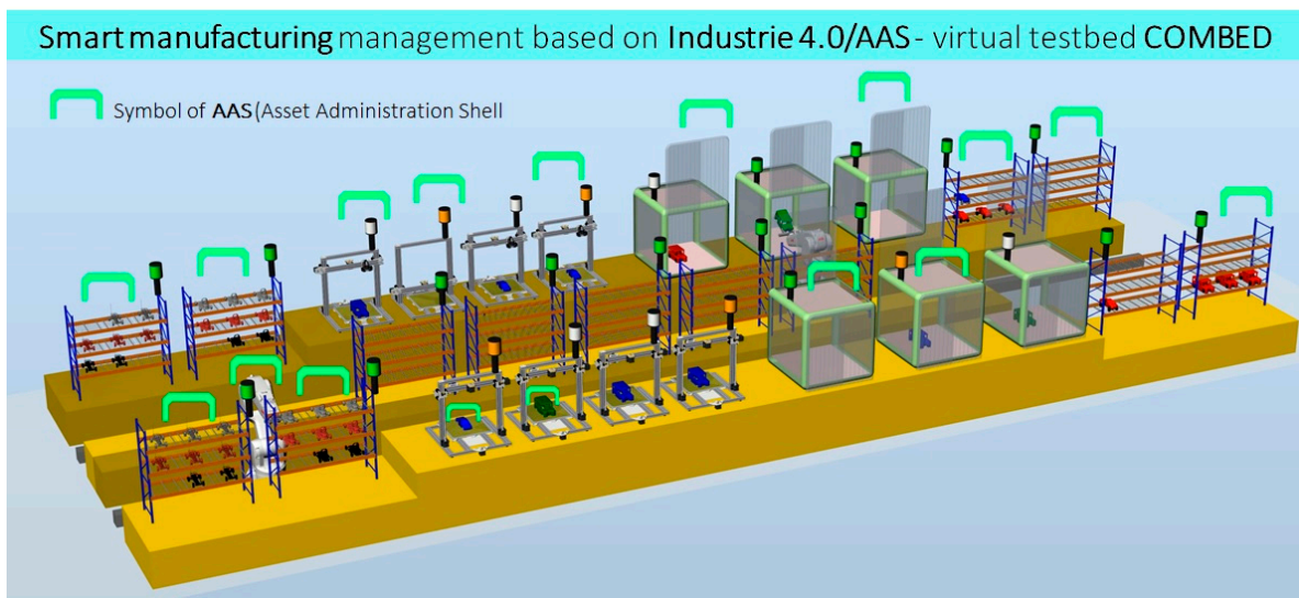
Figure 7. The virtual production segment (COMBED) introduced at the 2019 International Engineering Fair in Brno, the Czech Republic.
