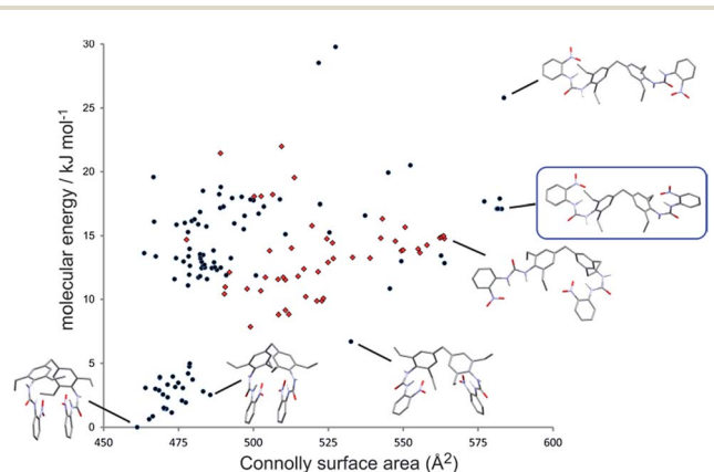
Fig. 4 Conformational landscape of gelator 2 . Each point represents the calculated (DFT-D) energy and Connolly surface area of a predicted conformer. Selected conformers are shown, with all hydrogen atoms hidden for clarity, apart from the urea hydrogens. Red points show conformations with one urea group in the anti-anti conformation. No conformations with both ureas in the anti-anti conformation are found in this energy range. The predicted most likely conformation, as a balance of intramolecular energy and extendedness, is enclosed in a blue box.
