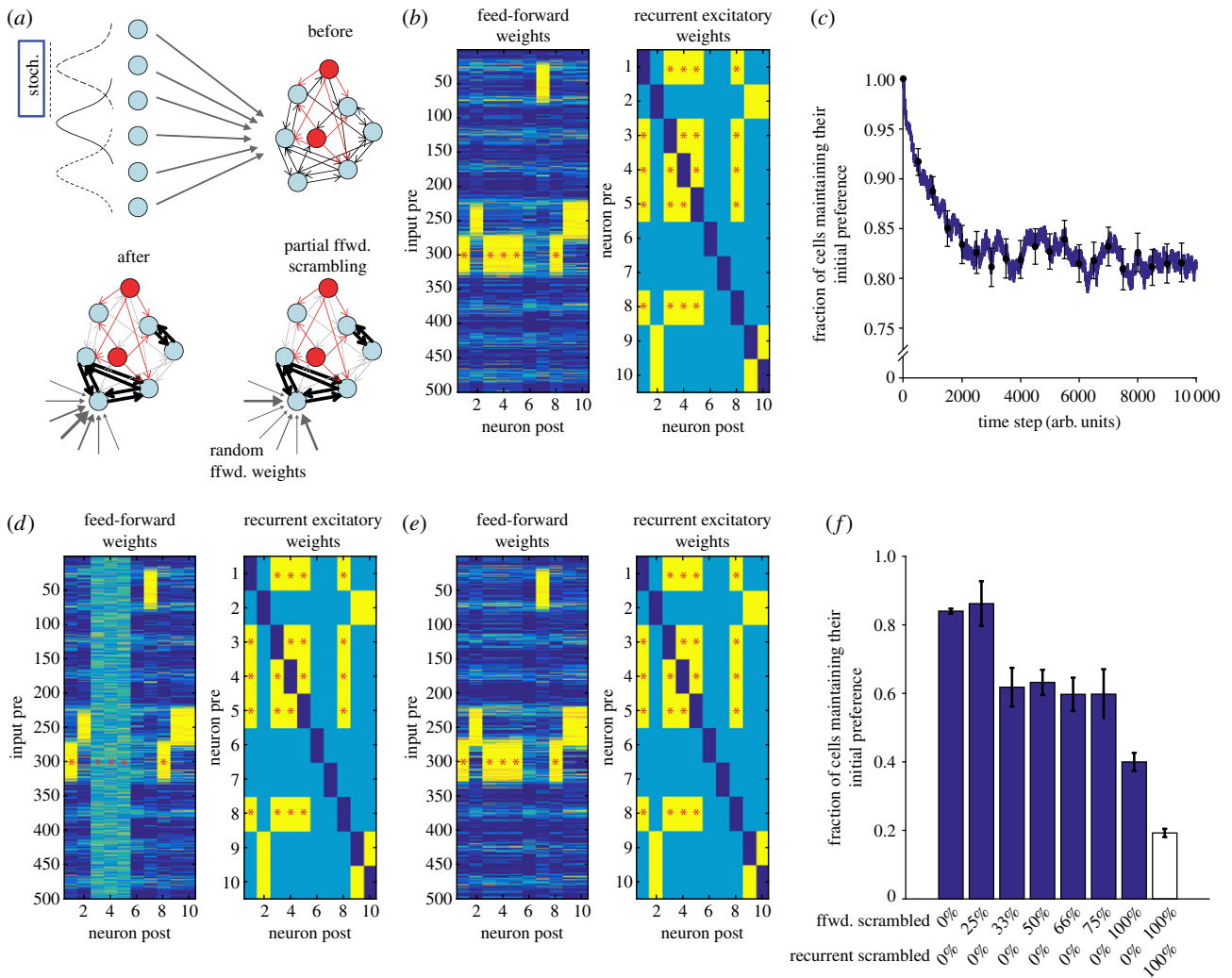
Figure 3. Model of a plastic microcircuit. (a) A densely interconnected network of 10 excitatory (light blue) and three inhibitory neurons (red) receives feed-forward (fwd) inputs from 500 Poisson spike trains with a Gaussian profile of firing rates. The centre of the Gaussian was shifted randomly to one out of 10 possible locations in stimulus space every model iteration (schematic network before (right) and after 10 000 model iterations (bottom left); see detailed methods and parameters in Clopath et al. [91]). (b) Network structure after 10 000 iterations of the model. Mean feed-forward weights (left) and recurrent excitatory weights (right) averaged over 1000 steps. The clustering of feed-forward weights (left) indicates that the neurons developed individual stimulus preferences. These ‘receptive fields’ were expressed as strong synaptic weights of the feed-forward inputs corresponding to one of the 10 stimulus positions (synaptic weights from weak, blue, to strong, yellow). The recurrent weights (right) were classified as weak (less than two-thirds of the maximal weight, light blue) or strong (more than two-thirds of the maximal weight, yellow). The diagonal is dark blue, as autaptic connections are not allowed in the model. Red asterisks indicate a recurrently connected example ensemble with similar receptive fields (cells 1, 3, 4, 5 and 8). (c) Baseline stability of the model. After the first 10 000 iterations of the model, it was allowed to continuously evolve over 10 000 further time steps. The similarity to the state after the first 10 000 steps decreased initially, but then plateaued. The model therefore did not show overt drift (cf. figure 1b). (d) As a perturbation, the feed-forward connections to three (cells 3, 4, 5) out of the five cells in the co-tuned example ensemble in (b) (red asterisks) were set to random values (see (a), bottom right). (e) The network converged back from the perturbation (10 000 further time steps). The initial receptive fields were recovered. (f) Fraction of cells selective to the same feature before and after perturbation for different degrees of perturbation. In all ensembles with at least two co-tuned cells, feed-forward inputs were scrambled for a variable fraction of the ensemble neurons: blue bars: randomized feed-forward inputs of a certain percentage of ensemble cells; white bar: all feed-forward and all recurrent weights were set to their random initial values. (Mean: average over 100 trials; error bars: standard deviation of the mean.)
