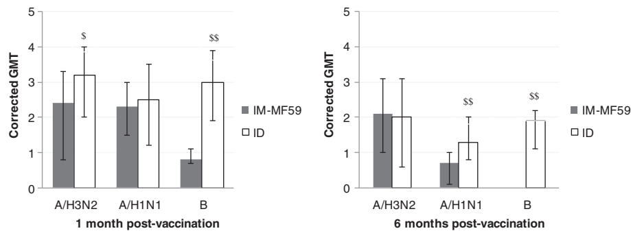
Figure 1 One and 6 months post-vaccination GMT against the three 2011-12 influenza vaccine components adjusted according to pre-vaccination titers. $: p < 0.05 ; $$: p < 0.01 comparing the two vaccine groups.
