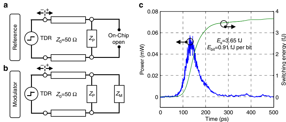
Figure 3 | Energy consumption. (a) The electrical setup for the time domain reflectometry (TDR) reference measurement, configured for measuring the reflected voltage ( V_{\bar{r}} ) from the open-ended on-chip pads ( Z_p ). (b) The electrical setup for the TDR reference and modulator measurement, configured for measuring the reflected voltage ( V_{\bar{r}M} ), from the modulator load ( Z_M ) and identical on-chip pads ( Z_p ). The TDR input and reflected TDR output directions are depicted with + and - signs. (c) The TDR measurement of the electro-optic modulator power consumption and switching energy for a 0.5V_{pp} AC-coupled drive.
