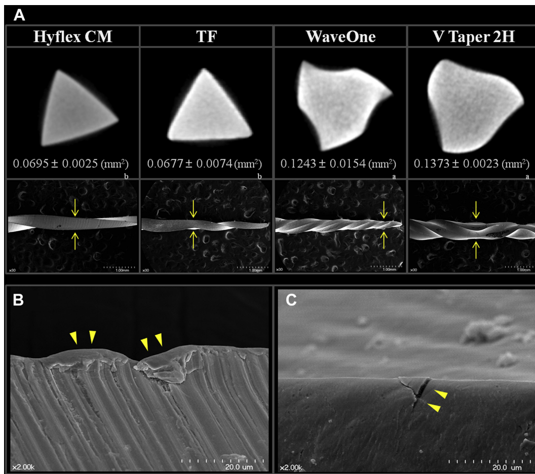
Figure 2 (A) Upper, cross-section images and the cross-sectional area ( \text{mm}^2 ) at a 3-mm level from the apical tip of each instrument. Microcomputed tomographic images. Lower, Scanning electron microscope images showing flute deformation (unwinding, arrow) of each instrument after canal preparation ( \times 30 ); (B) scanning electron microscope images showing roll over in WaveOne (arrowheads); (C) scanning electron microscope images showing roll over in microcrack in V Taper 2H (arrowheads) found at the deformed flute area of each instrument ( \times 20,000 ). Values with the same lowercase superscript letter are not significantly different ( P > 0.05 ). TF = Twisted File.
