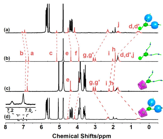
Figure 2. ^1\text{H} NMR titration of DAB with \beta -CD and CB[6] in the molecular self-assembling process.
