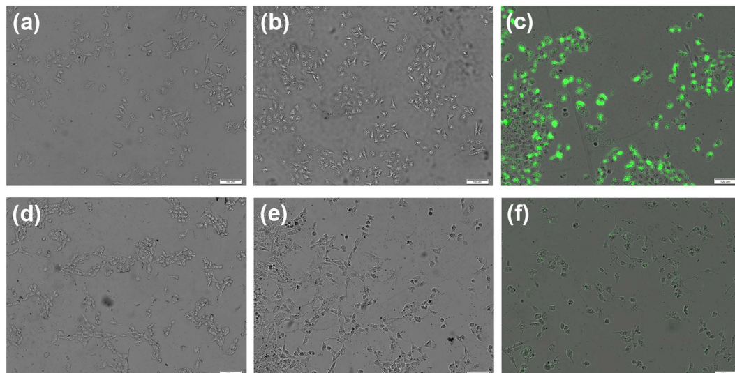
Figure 6. Selective uptake of FAM-siRNA by the supramolecular complexes and assembly. Fluorescence microscopic images of (a–c) PC-3 and (d–f) NIH3T3 cells incubated with FAM-siRNA containing (a,d) medium, (b,e) the ADA-HACD complex, and (c,f) the CB[6]-ADA-HACD assembly for 5 h.
