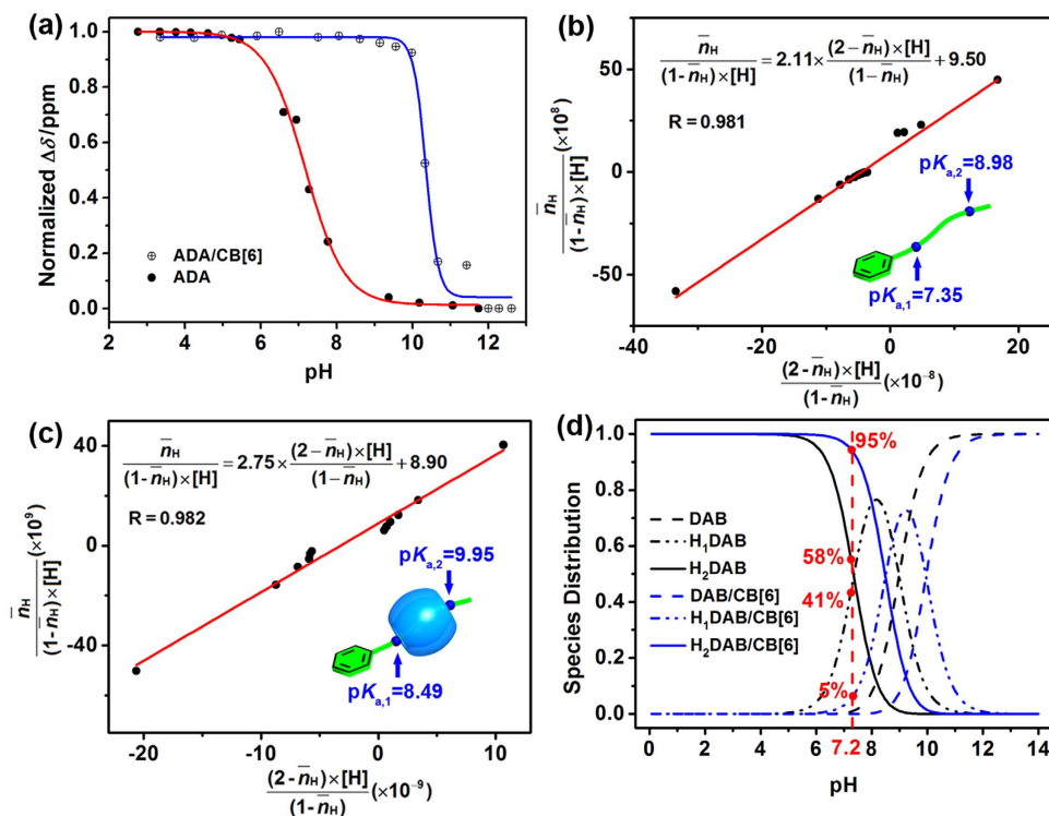
Figure 3. Supramolecular pK_a shift of DAB–CB[6] complex. (a) ^1\text{H} NMR titration curves for free ADA and ADA–CB[6] complex by monitoring \text{H}_f proton (see Fig. 1) upon variations in pH in aqueous solutions at 25 °C, which revealed a different degree of protonation induced by the complexation of ADA with CB[6] ([ADA] = 0.5 mM and [CB[6]] = 1.0 mM); for the original data, see Supplementary Fig. S29; potentiometric fitting curve and pK_a values calculation of (b) DAB and (c) DAB–CB[6] system ([DAB] = 0.5 mM and [CB[6]] = 1.0 mM); (d) pH-dependent species distribution plot for the DAB–CB[6] system. The distributions were obtained using the calculated pK_{a,1} and pK_{a,2} values. The H 1 DAB and H 2 DAB indicate the singly and doubly protonated species of DAB, respectively.
