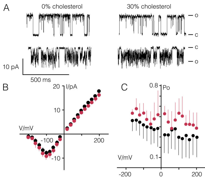
Figure 2. Impact of cholesterol in phosphatidylcholine bilayers on Kcv S function. (A) Representative channel fluctuations of Kcv S at +120 mV (top) and -120 mV (bottom) in a pure DPhPC bilayer (0% cholesterol) and in a DPhPC bilayer with 30 mol% cholesterol. Closed (C) and open (O) levels are indicated. (B and C) Open channel current/voltage (I/V) relations (B) and P O /V relations (C) in the absence (black) and presence of 30 mol% cholesterol (red). Data are mean ± SD of n = 10 (0% cholesterol) and n = 4 (30 mol% cholesterol) independent measurements.
