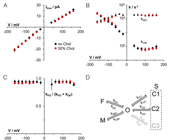
Figure 3. Effect of 30 mol% cholesterol in DPhPC bilayers on the true current and fast gating in Kcv NTS analyzed with β distributions. (A) True single-channel current I true . (B) Rate constants of channel closing (k OM ) and opening (k MO ) of sub-millisecond gating (O-M gating). (C) Gating factor of the microsecond gating (O-F gating) k FO /(k FO + k OF ), i.e., the open probability of O-F gating. (D) Gating model used for analysis. The rate constants of gating between state O (open) and the short closed states F and M were analyzed with extended β distributions, the gating related to the longer closed states (C1, C2, and for Kcv S additionally C3) with dwell-time analysis (see main text). Data points represent mean ± SD in A and C and geometric mean ± geometric SD in B. Six and three independent experiments were without and with cholesterol, respectively. At lower voltages, some data points are missing because the signal-to-noise ratio here was not sufficient for a reliable fit in all experiments. Chol, cholesterol.
