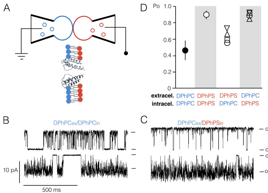
Figure 9. Recording of Kcv 5 in asymmetrical bilayers. (A) Principle of the contact bubble bilayer method. Glass pipettes filled with liposomes of different lipids (red and blue circles) are immersed in an oil bath. By applying pressure to the pipettes PL monolayer bubbles with different lipid (red or blue), compositions are produced in the oil bath. At the contact point, the two monolayers form a bilayer in which the two leaflets are made from different PLs. Blowup: After insertion of the channel protein into the asymmetric bilayer, the cytosolic and extracellular sides will be exposed to different PLs. (B and C) Representative channel fluctuations at +120 mV (top) and -120 mV (bottom) in a symmetrical DPhPC bilayer (in B) and in an asymmetrical bilayer with DPhPS on the cytosolic side of the channel (in C). Closed (C) and open (O) levels are indicated. (D) Mean P O values for single-channel recordings of Kcv 5 in symmetrical or asymmetrical bilayers with DPhPC and DPhPS on the cytosolic or external side. Data are mean values ± SD (n = 4) for recordings in symmetrical bilayers and values from individual measurements (triangles, square, circle) for asymmetrical bilayers.
