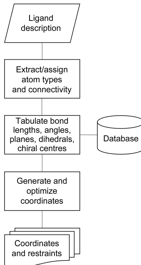
Figure 1 Schematic of the dictionary-generation process.
