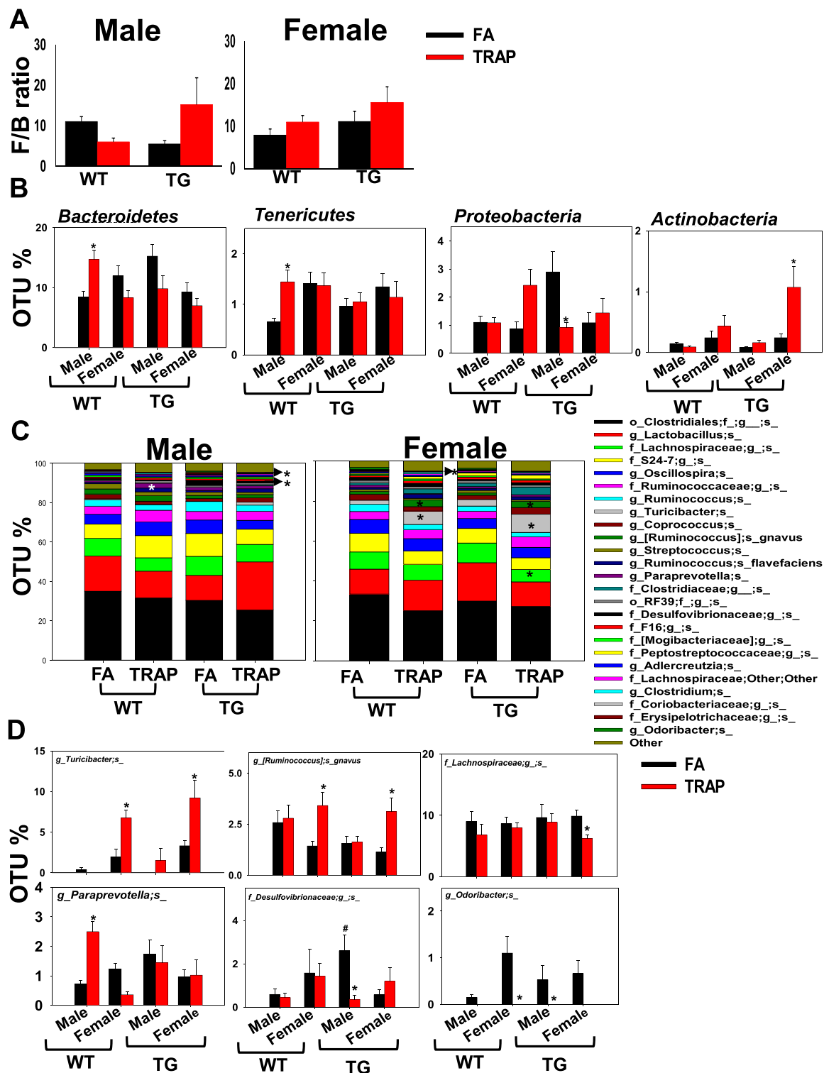
Fig. 3. (A) F/B ratio in male (left) and female (right) WT and TgF344-TG rats after 14 months exposure to FA or TRAP (n = 5–6 per group). (B) Differentially regulated bacterial phyla (L2) by TRAP after 14 months exposure (asterisks [*] represent statistically significant differences as compared to the FA-exposed group of the same sex and genotype, p < 0.05 ). Statistical significance was determined using two-way ANOVA followed by Tukey’s post hoc test. (C) Proportion of bacterial species (L7) observed in FA and TRAP exposed male and female rats. (D) Differentially regulated bacterial species (L7) in female and male rats after 14 months exposure to TRAP. Asterisks (*) represent statistically significant differences when compared with different exposure of similar sex and genotype ( p < 0.05 ) whereas pound (#) symbolize statistically significant differences among different genotypes of similar sex and exposure ( p < 0.05 ). Data was analyzed using two-way ANOVA followed by Tukey’s post hoc test.
