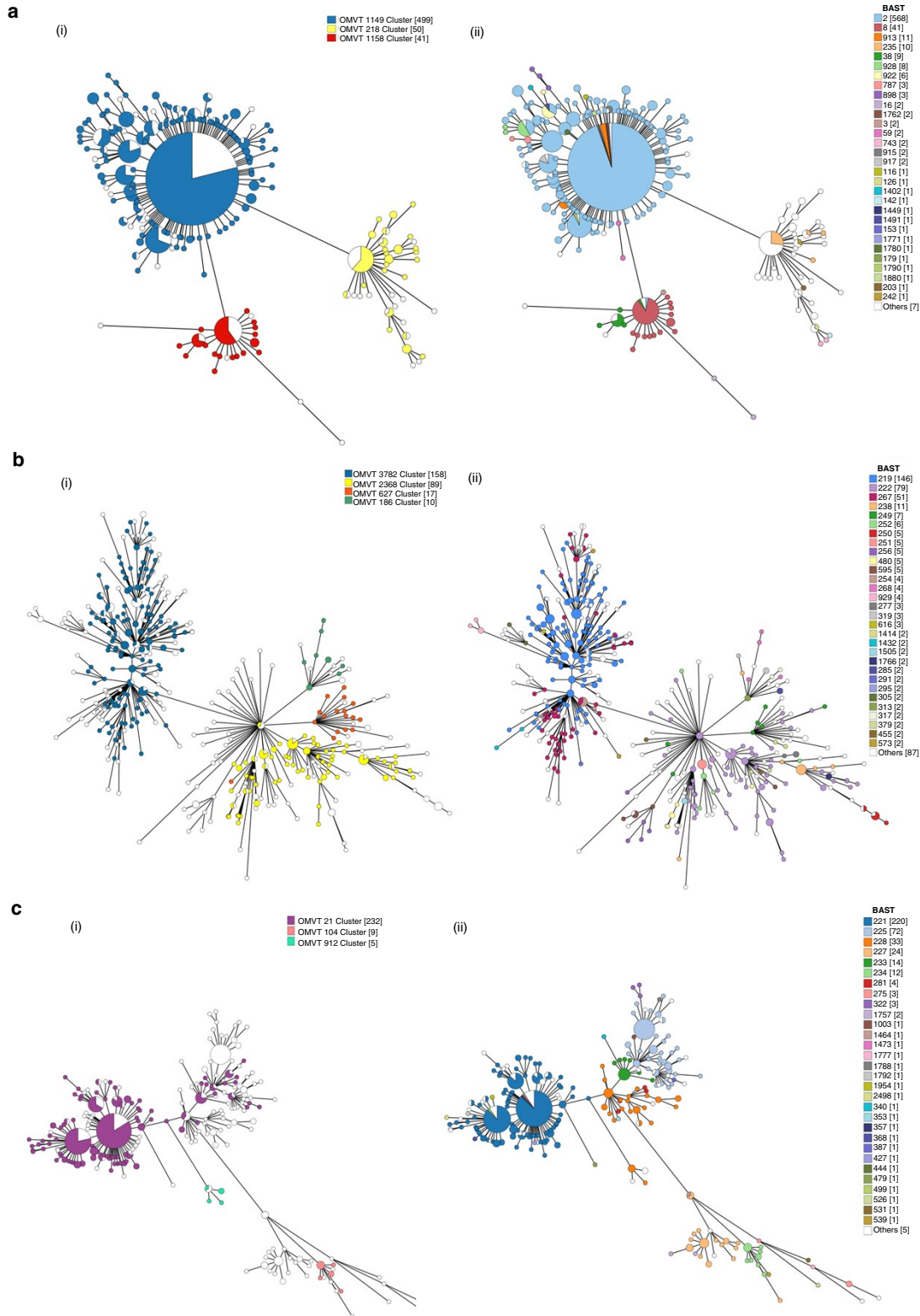
Figure 7. Outer Membrane Vesicle peptide Typing (OMVT) clusters and association with Bexsero® Antigen Sequence Types (BASTs). (a) Clonal complex 11 (cc11) isolates (n=777) were analysed using the OMVT scheme. (i) Clusters of OMVTs that match 18 loci to the central OMVT are shown. Cc11 has 3 OMVT clusters, 1149, 218 and 1158. OMVT 1149 cluster represents lineage 11.2, OMVT clusters 218 (yellow) and 1158 (red) represent lineage 11.1. (ii) OMVT clusters are coloured by BASTs, demonstrating the strong non-overlapping association of BASTs with OMVT clusters. Unfilled nodes represent incomplete data, so a profile could not be assigned. (b) Cc269 isolates (n=500) were analysed using the OMVT scheme. (i) Cc269 has 4 OMVT clusters. (ii) OMVT clusters are coloured by BAST. (c) Cc23 isolates (n=459) were analysed using the OMVT scheme. (i). Cc23 has 3 OMVT clusters. (ii) OMVT clusters are coloured by BAST.
