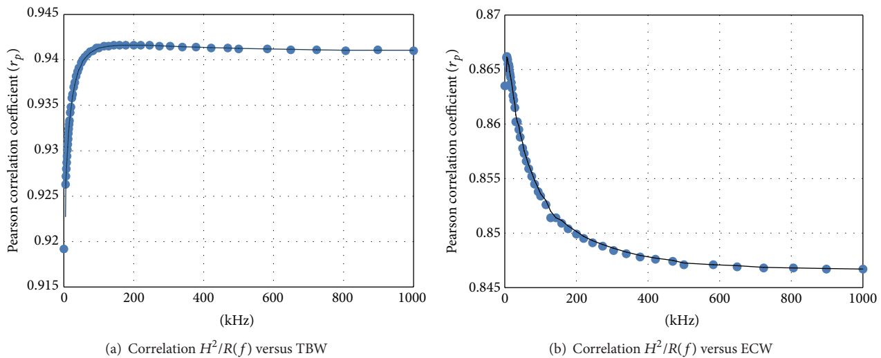
FIGURE 2: Correlation of impedance quotients H^2/R (kHz) and estimated body fluids at different frequencies. Total body water in panel (a) and extracellular fluid in panel (b).
