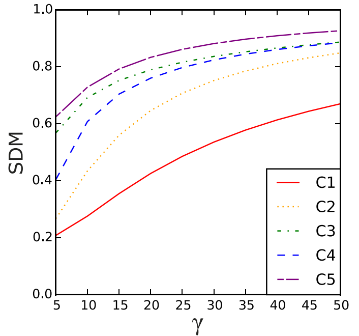
Figure 3. Predicted difficulty in the conditions of Alfonso-Reese, Ashby, and Brainard (2002) as a function of the \gamma parameter of the Striatum Difficulty Measure.
