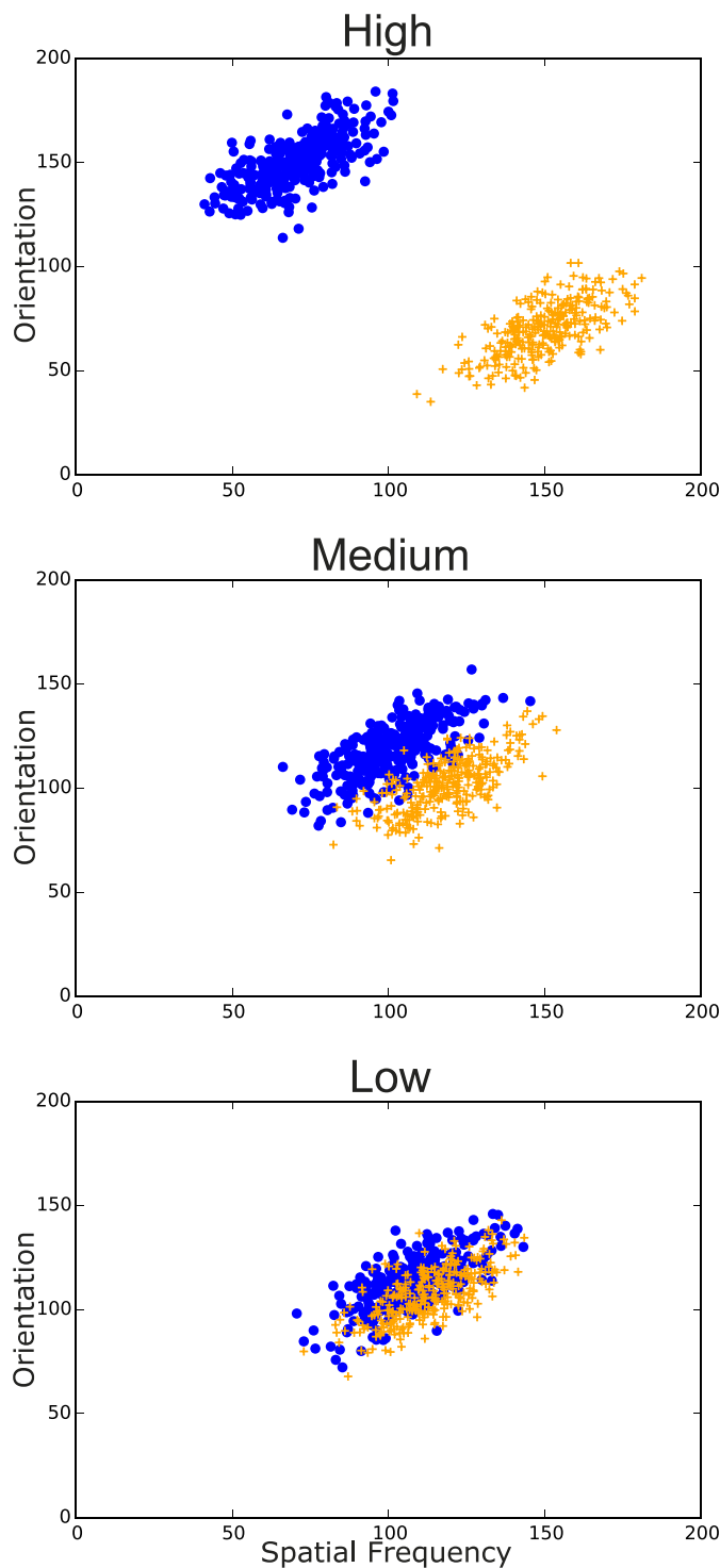
Figure 6. Ell and Ashby (2006) category structures. In each case, categories were created by random sampling from a bivariate normal distribution. All distributions had identical variance-covariance matrices. The three conditions varied the intermean distance to create high, medium, and low class separation.
