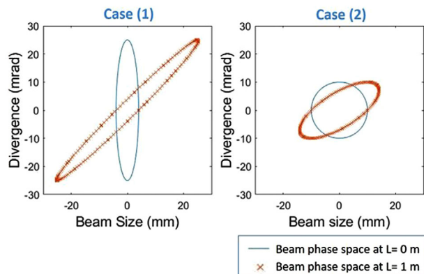
FIGURE 1 Evolution of the phase space in transverse plane from the start until the end of a 1 m long beam pipe (beam emittance is 100 \pi^* \text{mm}^* \text{mrad} )
