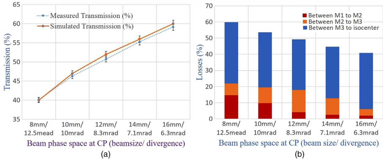
FIGURE 5 (a) Beam transmission through gantry (simulation and measured) for transporting 100 \pi^*mm^*mrad through gantry with different beam parameters at the CP with different imaging factors as shown in Figure 4. (b) Beam losses distribution (measured) along the different parts of the gantry while transporting 100 \pi^*mm^*mrad emittance with different phase space at the CP
