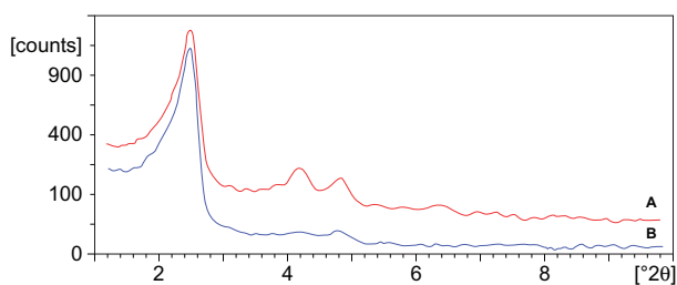
Figure 2 X-ray diffraction patterns of PF-MCM-41 (A) and AuCl 3 @PF-MCM-41 (B). The patterns exhibit a high intensity (100) reflection within the 2\theta range of 2^\circ – 3^\circ . The similar d_{100} spacing values confirmed the maintenance of two-dimensional hexagonal mesoporous structures ( P_{6mm} ) of MCM-41 after introducing complexes.
