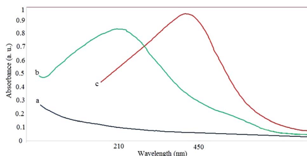
Fig. 1 Absorption spectra of plant extract (a), SPIONPs (b) and AgNPs (c).
