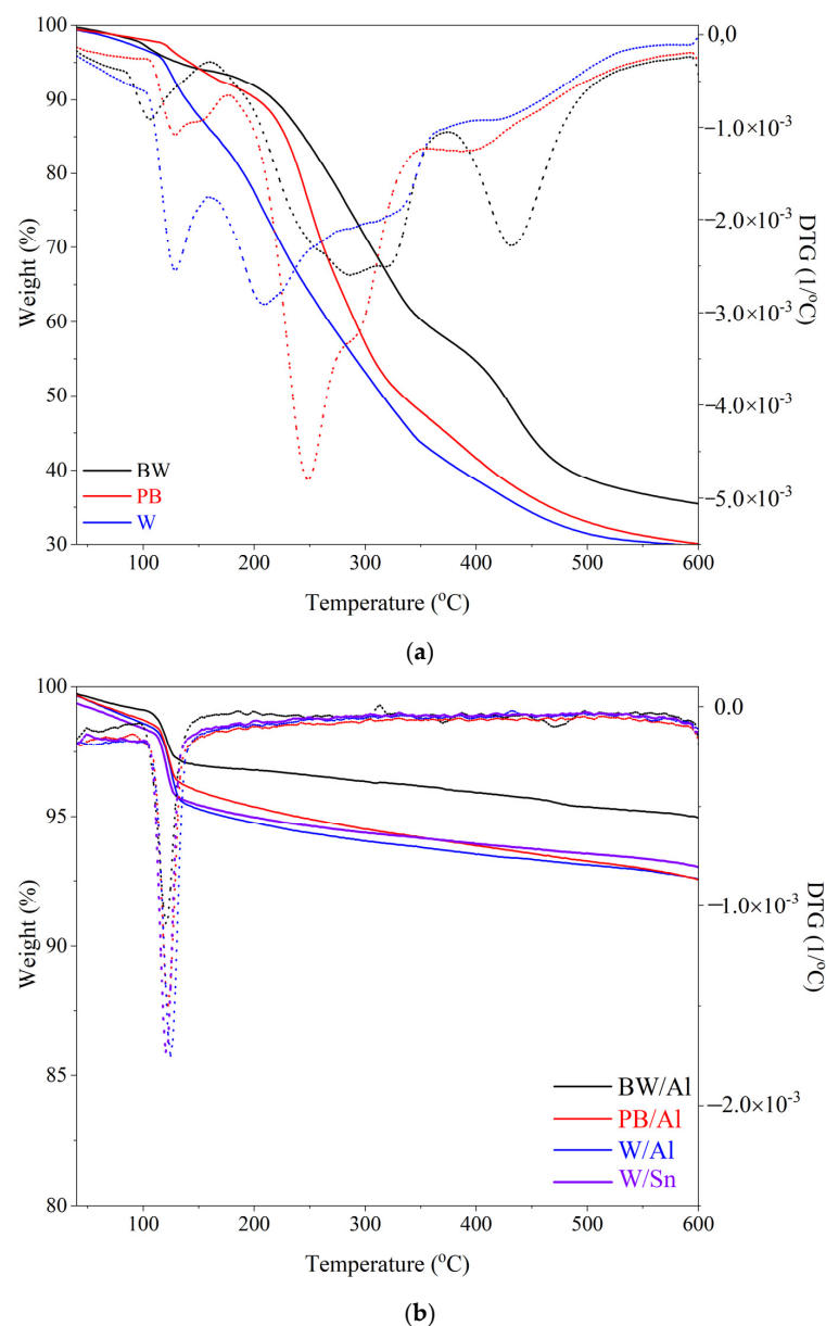
Figure 5. Thermogravimetric curves (TG/DTG) obtained for: natural dyes (a) and lake pigments (b).
