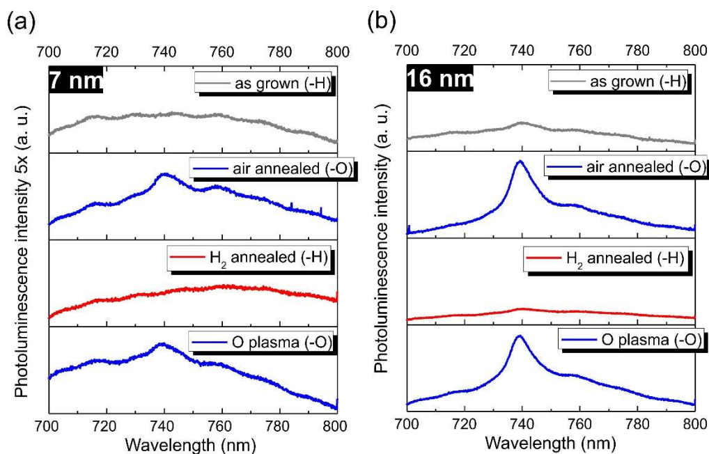
Figure 5. SiV PL data of 7 nm (a) and 16 nm (b) NCD2 films in dependence on the surface chemistry variation. The specific treatments are mentioned in the legends for clarity.
