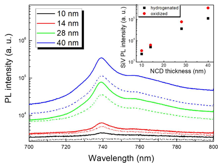
Figure 2. Semi-log plots of photoluminescence (PL) spectra showing shallow silicon vacancy (SiV) PL evolution of plasma-hydrogenated H1-NCD1 films (dotted lines) and air-annealed, i.e., oxidized, O2-NCD1 films (full lines) in dependence on increasing NCD film thickness. The inset shows SiV PL intensity in semi-log scale as a function of NCD film thickness and the NCD surface chemistry.
