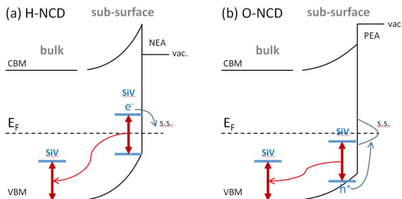
Figure 4. Schematic model of the proposed mechanism for the opposite SPV and its decrease with increasing NCD layer thickness together with increasing PL intensity for the hydrogenated (a) and oxidized (b) NCD surfaces.
