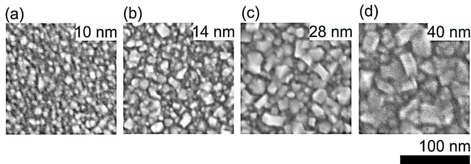
Figure 1. Representative scanning electron microscopy (SEM) images of ultra-thin nanocrystalline diamond (NCD) films having thicknesses of 10 nm (a), 14 nm (b), 28 nm (c), and 40 nm (d).
