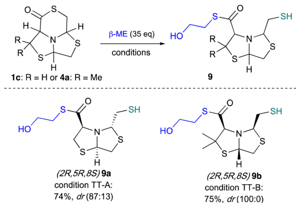
Fig. 8 Thiolysis of \delta -thiolactones 1c and 4a . Condition TT-A: Gly (1.2 eq.), MeCN : DMF (3 : 1), gave: 9a 74%, dr (87 : 13); condition TT-B: Gly (1.2 eq.), H 2 O : AcOEt (1 : 1), gave: 9b 75%, dr (100 : 0).
