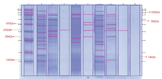
Figure 2. Results of electrophoresis. kDa = molecular weight in kilo dalton, lane 1 = marker, lane 2 = standard (planktonic), lane 3 = glucose-induced pellet, lane 4 = glucose-induced biofilm, lane 5 = lactose-induced pellet, lane 6 = lactose-induced biofilm, lane 7 = soy protein-induced pellets, lane 8 = soy protein-induced biofilm, lane 9 = iron-induced pellet, lane 10 = iron-induced biofilm.
