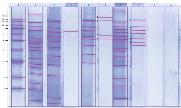
Figure 1. Results of electrophoresis. KDa = weight of molecules in kilo dalton, lane 1 = marker, lane 2 = standard (planktonic), lane 3 = glucose-induced pellet, lane 4 = glucose-induced biofilm, lane 5 = lactose-induced pellet, lane 6 = lactose-induced biofilm, lane 7 = soy protein-induced pellets, lane 8 = soy protein-induced biofilms, lane 9 = substance-induced pellets, lane 10 = iron-induced biofilms.
