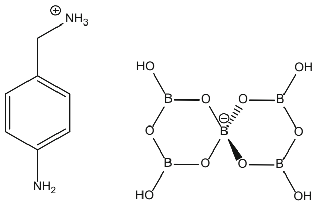
Fig. 1 Schematic representation of the cation and anion present in [ p -H 2 NC 6 H 4 CH 2 NH 3 ][B 5 O 6 (OH) 4 ] \cdot 1/2H 2 O ( 1 )
