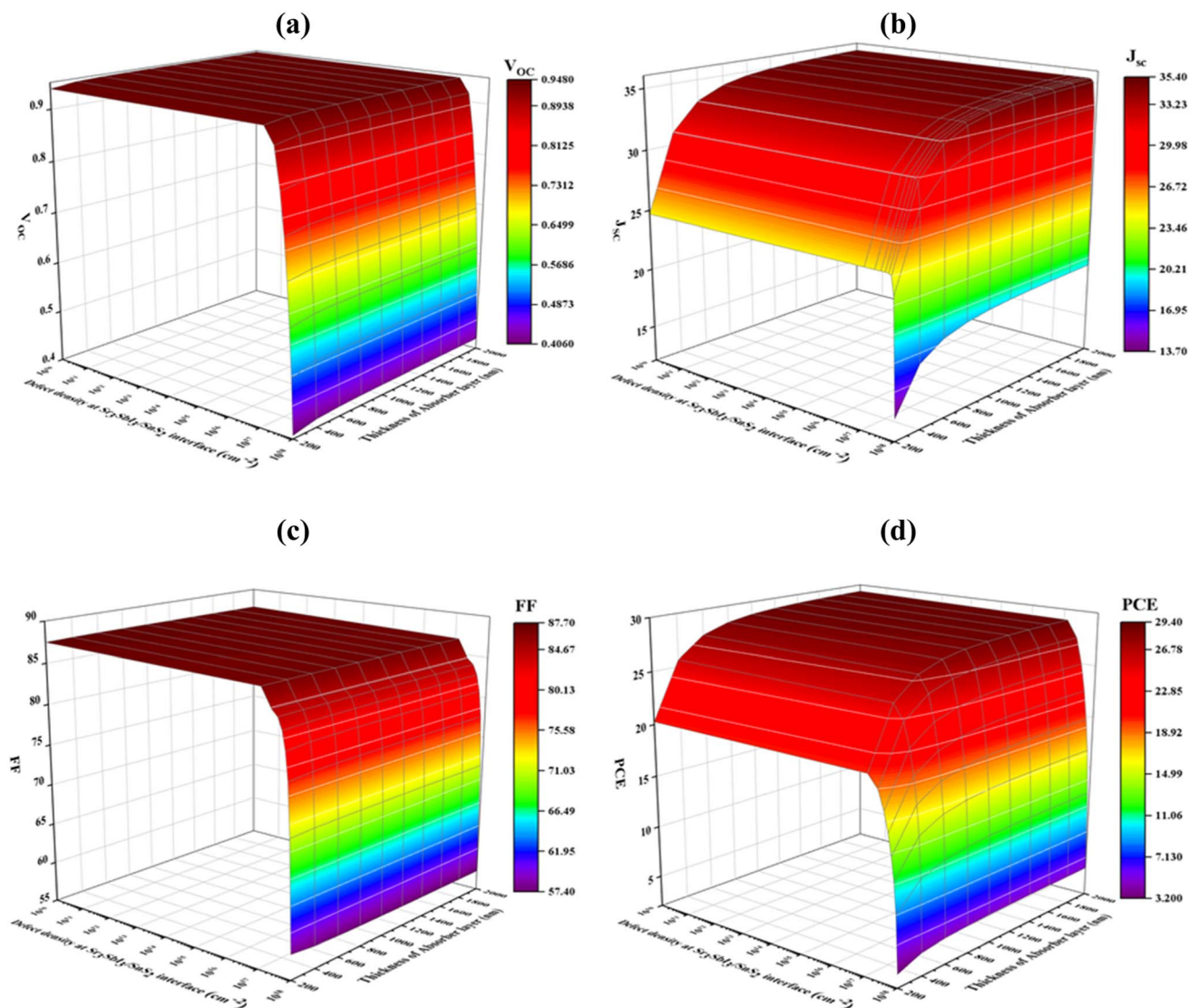
Fig. 8 Effects of thickness of absorber and interface ( \text{Sr}_3\text{SbI}_3/\text{SnS}_2 ) defect density variations on photovoltaic parameters of (a) V_{\text{OC}} (b) J_{\text{SC}} (c) FF and (d) PCE.
