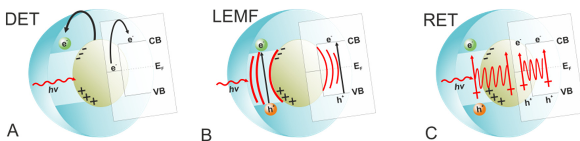
Figure 20. Various mechanism of plasmon energy transfer from metal to the semiconductor. (A) Direct electron transfer (DET) of hot electrons, (B) local electromagnetic field enhancement (LEM) of the semiconductor charge separation process, (C) resonant energy transfer (RET).
