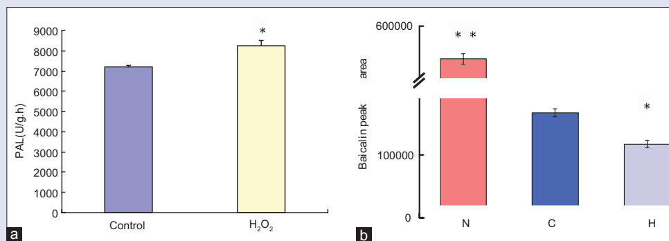
Figure 4: Effects of H 2 O 2 on activities of phenylalanine ammoniylase, UDP-glucuronate baicalein 7-O-glucuronosyltransferase, and β-glucuronidase. (a) The effect of H 2 O 2 on the phenylalanine ammoniylase, H 2 O 2 increasing the activity of phenylalanine ammoniylase significantly. (b) is integrate effect of H 2 O 2 on UDP-glucuronate baicalein 7-O-glucuronosyltransferase and β-glucuronidase, "N", "C", and "H" stands for denatured enzymes, control with normal enzyme, treated with H 2 O 2 respectively. Compared with denatured enzymes, the baicalin content in the control and the H 2 O 2 decreased remarkable, but compared with the control, the H 2 O 2 decreased significantly
