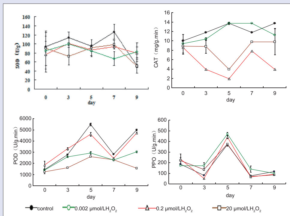
Figure 2: Effects of H 2 O 2 on activities of superoxide dismutase, catalase, peroxidase, and polyphenol oxidase. With 0.002 \mu mol/L, 0.2 \mu mol/L H 2 O 2 , and 20 \mu mol/L H 2 O 2 , superoxide dismutase, catalase and peroxidase activities suffered, particularly catalase, indicating under stress situation, anti-oxidative enzyme system fails to quench directly excessive reactive oxygen species in the plant cell. The activity of polyphenol oxidase was driven up slightly, showing flavones may be take important role in smoothing reactive oxygen species under heavy stress situation. The performance was repeated 3 times
