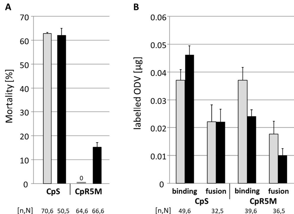
Figure 3. Mortality and results of fluorescence dequenching assays of CpS and CpR5M per os infected with labeled ODV. L4 larvae were orally infected with 2.4 \mu\text{g} of labeled ODV of CpGV-M (gray) or CpGV-S (black). (A) Abbott-corrected mean mortality and standard errors (error bars) were recorded 7 days post-infection. (B) Amount of labeled ODV bound or fused with midgut epithelial cells; dissection of midgut epithelial cells was undertaken 1 h post-infection. The total number of tested individuals (n) and number of independent replicates (N) are given below the chart.
