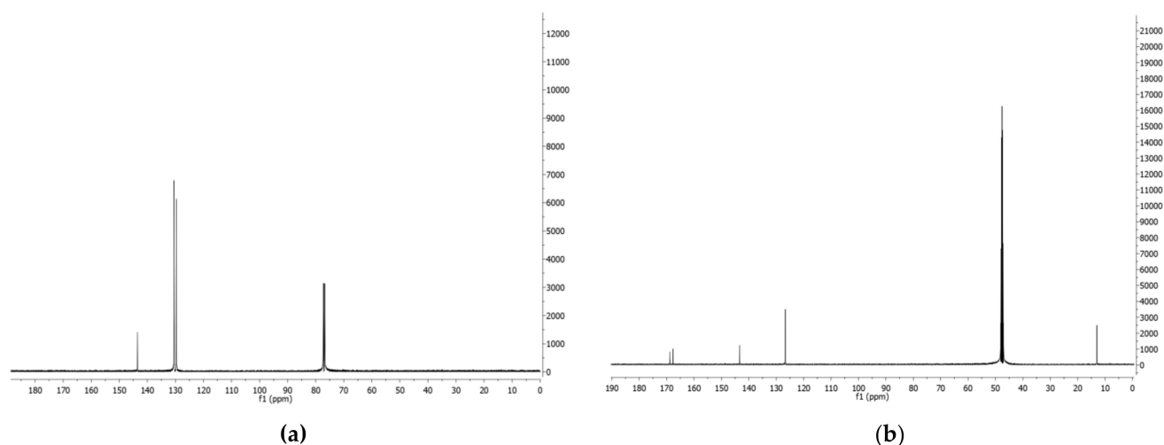
Figure 4. (a) ^{13}\text{C} -NMR spectrum of phenazine (1) recorded in \text{CDCl}_3 at 125 MHz; (b) ^{13}\text{C} -NMR spectrum of mesaconic acid (2) recorded in \text{CD}_3\text{OD} at 125 MHz.
