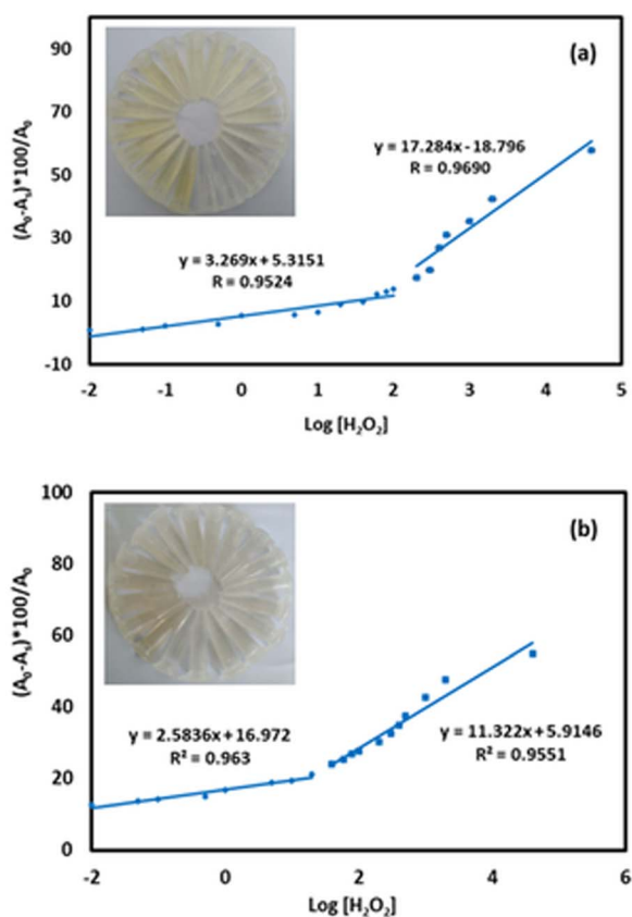
Fig. 4 Response changes plotted against the logarithm of H_2O_2 concentration: (a) AgNP1 (b) AgNP2.
