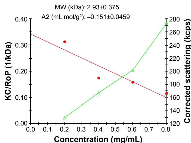
Figure 4 Debye plot of glutamine conjugated to dendrimer-G 2 .
