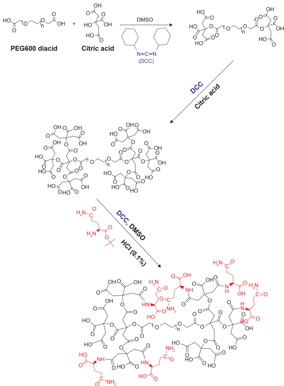
Scheme 1 The preparation routes of dendrimer-G 2 and glutamine conjugation. Abbreviations: DCC, N, N'-dicyclohexylcarbodiimide; DMSO, dimethyl sulfoxide.
