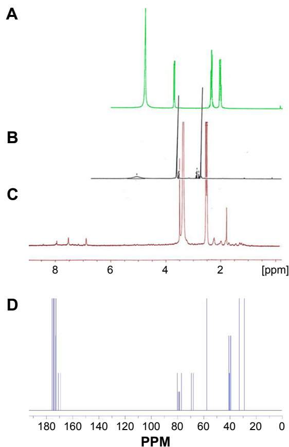
Figure 2 The 1 H-NMR spectrum of (A) glutamine, (B) dendrimer-G 2 , (C) dendrimer–glutamine, and (D) 13 C-NMR of dendrimer–glutamine.
