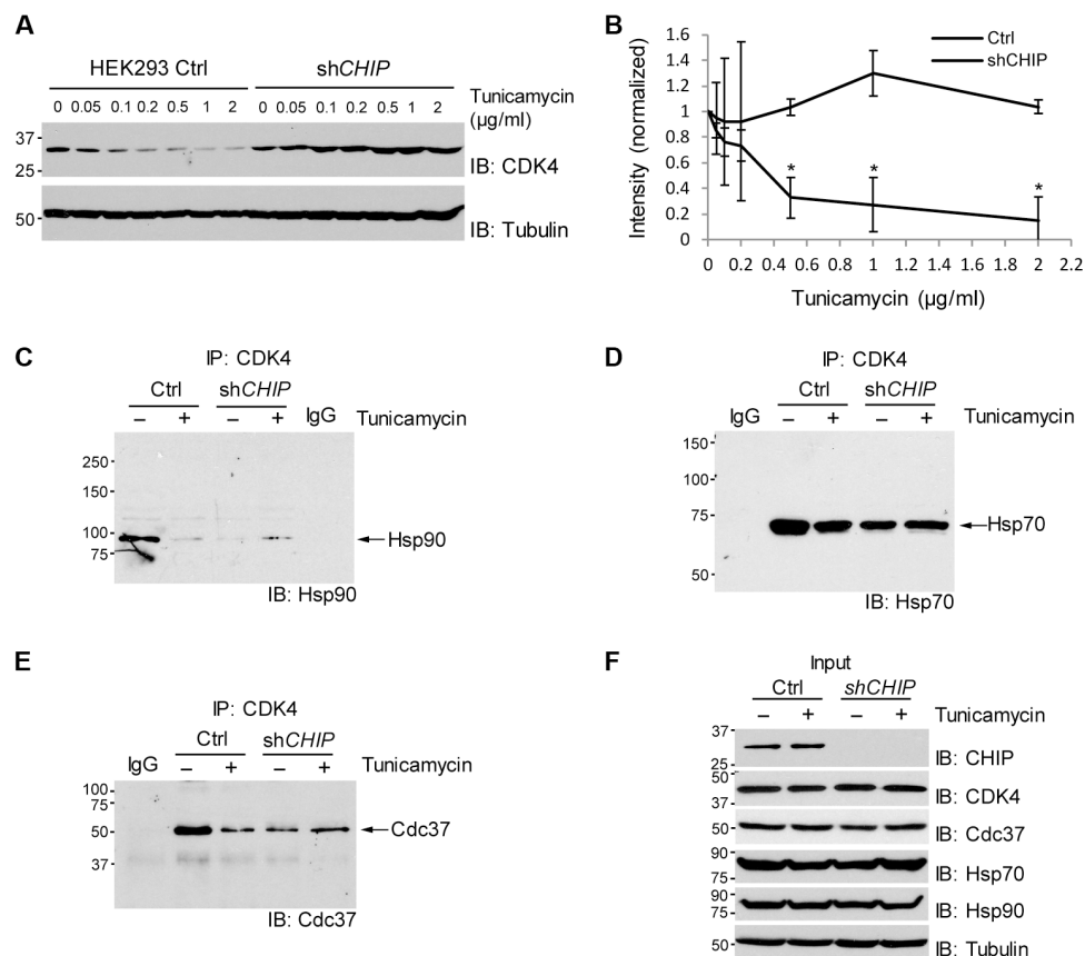
Fig. 10. ER stress-induced degradation of CDK4 is mediated by CHIP. (A) shCHIP abrogates down-regulation of CDK4 protein in HEK293 cells after treatment with tunicamycin. Cells were incubated for 72 hours with tunicamycin at the indicated concentrations and harvested for immunoblotting. (B) Quantification of CDK4 protein levels after normalization by the levels of tubulin. Data are means \pm SEM from three biological replicates, and the asterisks indicate statistical significance ( P < 0.05 ). (C) ER stress decreases association of CDK4 with Hsp90 in HEK293 control cells but not in shCHIP cells. (D) ER stress does not significantly affect CDK4 association with Hsp70. (E) ER stress decreases association of CDK4 with Cdc37 in HEK293 control cells but not in shCHIP cells. (C to E) Cells were incubated with tunicamycin (1 \mu g/ml) for 24 hours and then 10 \mu M MG132 was added to the medium, followed by incubation for an additional 1.5 hours. Cell lysates were immunoprecipitated (IP) with CDK4 antibody, followed by immunoblotting for the indicated proteins. IgG, negative control for IP with normal IgG. (F) The levels of the indicated proteins determined by direct immunoblotting using the cell lysates before IP.
