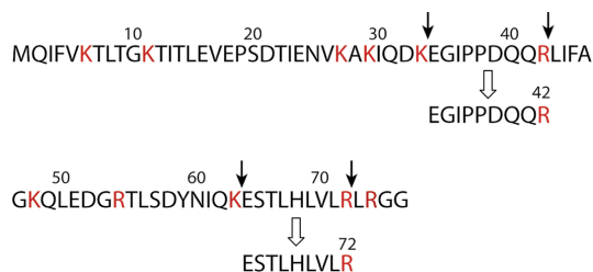
Fig. 11. Peptide sequence of wt UB and sites of trypsin digestion. Trypsin digests peptides immediately after Lys (K) or Arg (R) residues. Because of the mutations of R42E and R72E in xUB, trypsin would not cleave the xUB peptide at residues 42 and 72. Peptides with the sequence “EGIPPDQQR” and “ESTLHLVLR” are unique to trypsin digestion of wt UB.
