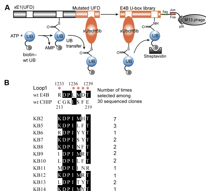
Fig. 1. Phage selection for the orthogonal xUbcH5b-xU-box pair for E4B. (A) wt UB labeled with biotin (biotin-wt UB) was activated by xUba1(UFD) and loaded on xUbcH5b. The U-box library of E4B was displayed on the surface of M13 phage. Phage displaying U-box mutants reactive with xUbcH5b were conjugated with biotin-UB and selected by binding to streptavidin. ATP, adenosine 5'-triphosphate; AMP, adenosine 5'-monophosphate. (B) Sequence alignment of U-box mutants of E4B from phage selection. Sites of randomized residues in the loop1 of the E4B U-box are marked by red asterisks. After five rounds of selection, 30 phage clones were sequenced; the alignment of the sequences showed that the phage library was converged to KB2 and other highly homologous clones.
