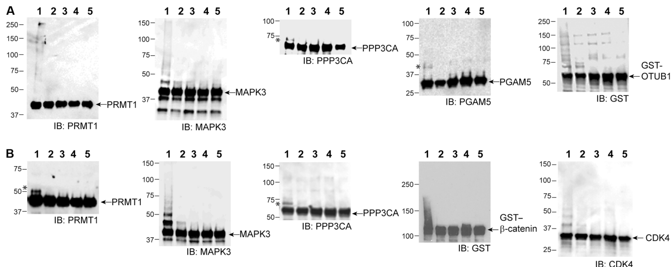
Fig. 5. In vitro assay to verify that E4B and CHIP catalyzed the ubiquitination of the substrates. (A) Ubiquitination of PRMT1, MAPK3, PPP3CA, PGAM5, and OTUB1 by wt UB through the wt Uba1-UbcH5b- \text{E4B} cascade (lane 1). In lanes 2, 3, 4, and 5, wt E4B, Uba1, UbcH5b, and wt UB were missing from the reaction mixture, respectively. GST, glutathione S-transferase. (B) Ubiquitination of PRMT1, MAPK3, PPP3CA, \beta -catenin, and CDK4 by wt UB through the wt Uba1-UbcH5b-CHIP cascade (lane 1). In lanes 2, 3, 4, and 5, wt CHIP, Uba1, UbcH5b, and wt UB were missing from the reaction mixture, respectively. Bands marked with asterisks were likely generated by monoubiquitinated substrates.
