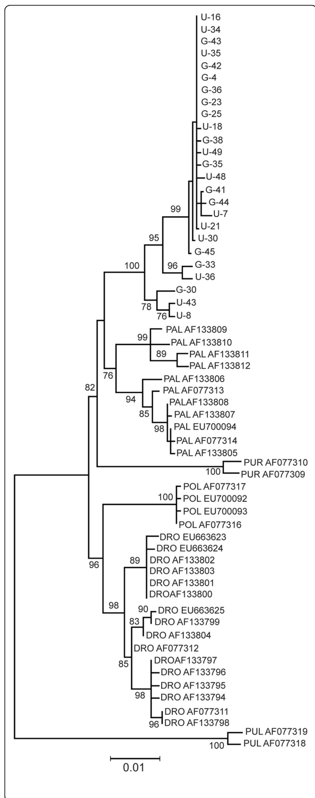
Fig. 2 Maximum likelihood tree of the stronglylenticrotid sea urchins bindin sequences. The tree is based on Kimura 2-parameter (K2P) model as the best-fitting model of substitution under the maximum likelihood criterion [66] for constructing an ML tree of the bindin sequences. The numbers at the nodes are bootstrap percent probability values based on 1,000 replications. The bindin sequences of Hemicentrotus pulcherrimus (AF077318 and AF077319) are used as outgroups. The specimens of S. intermedius are marked with letters "G" and "U". DRO = S. droebachiensis , PAL = S. pallidus ; POL = S. polyacanthus ; PUR = S. purpuratus ; PUL = Hemicentrotus pulcherrimus
