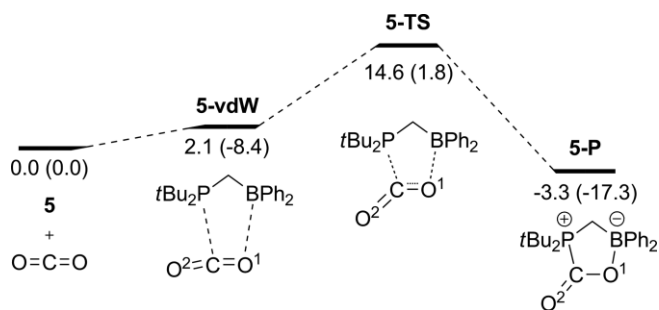
Figure 3. Relative \omega B97X-D/6-311G(d,p) Gibbs free energies (energy in brackets) in kcal mol -1 for the reaction of CO 2 and 5 .
