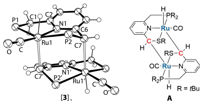
Figure 4. Two examples of dimeric MLC complexes. Left: molecular X-ray structure of [3] 2 (displacement ellipsoids are set at 50% probability, isopropyl groups on the phosphorus are omitted for clarity). [12] Selected bond lengths [Å]: Ru1-C7' 2.409(7), Ru1'-C7 2.403(7), P2-C7 1.797(6), C6-C7 1.456(8), C1-C2 1.489(9), C1-P1 1.842(6), P2'-C7' 1.803(6), C6'-C7' 1.449(8), C1'-C2' 1.55(1), C1'-P1' 1.843(6). Right: Milstein's Ru(PNS) dimer A . [18] Blue: Lewis acid; red: Lewis base.
