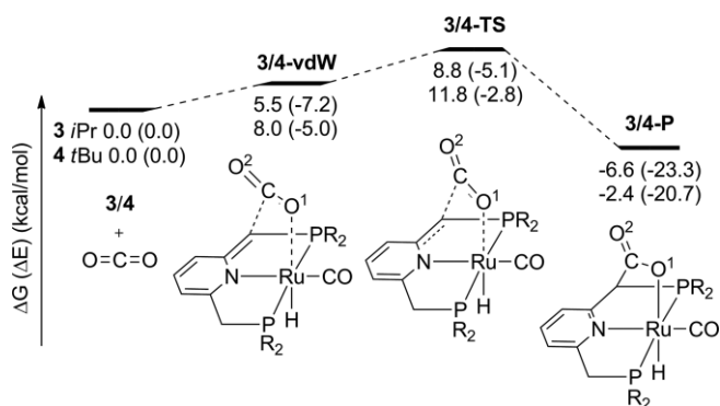
Figure 2. Relative \omega B97X-D/6-311G(d,p) Gibbs free energies (energy in brackets) in kcal mol -1 for the reaction of CO 2 and 3/4 .
