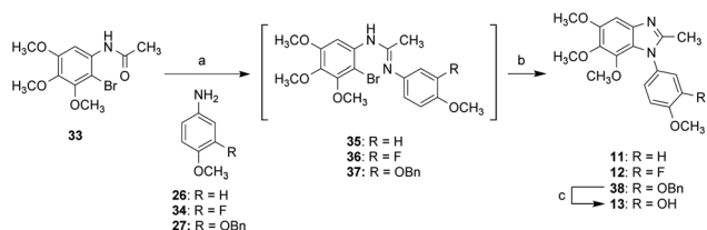
Scheme 4 Synthetic approaches to compounds 11–13: (a) for 35 and 37: POCl 3 , 26 or 27, toluene, 0 °C to 90 °C; for 36: triflic anhydride, 34, 2,6-lutidine, DCM, 0 °C to 50 °C; (b) CuI, 1,10-phenanthroline, K 2 CO 3 , ACN, reflux; (c) 10% Pd/C, H 2 , MeOH, rt.
