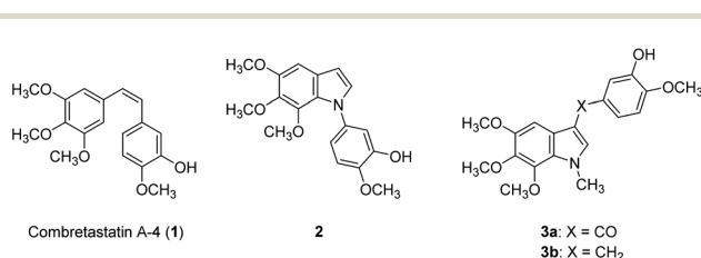
Fig. 1 Combretastatin A4 ( 1 , CA-4) and 5,6,7-trimethoxyindoles ( 2 and 3 ).
