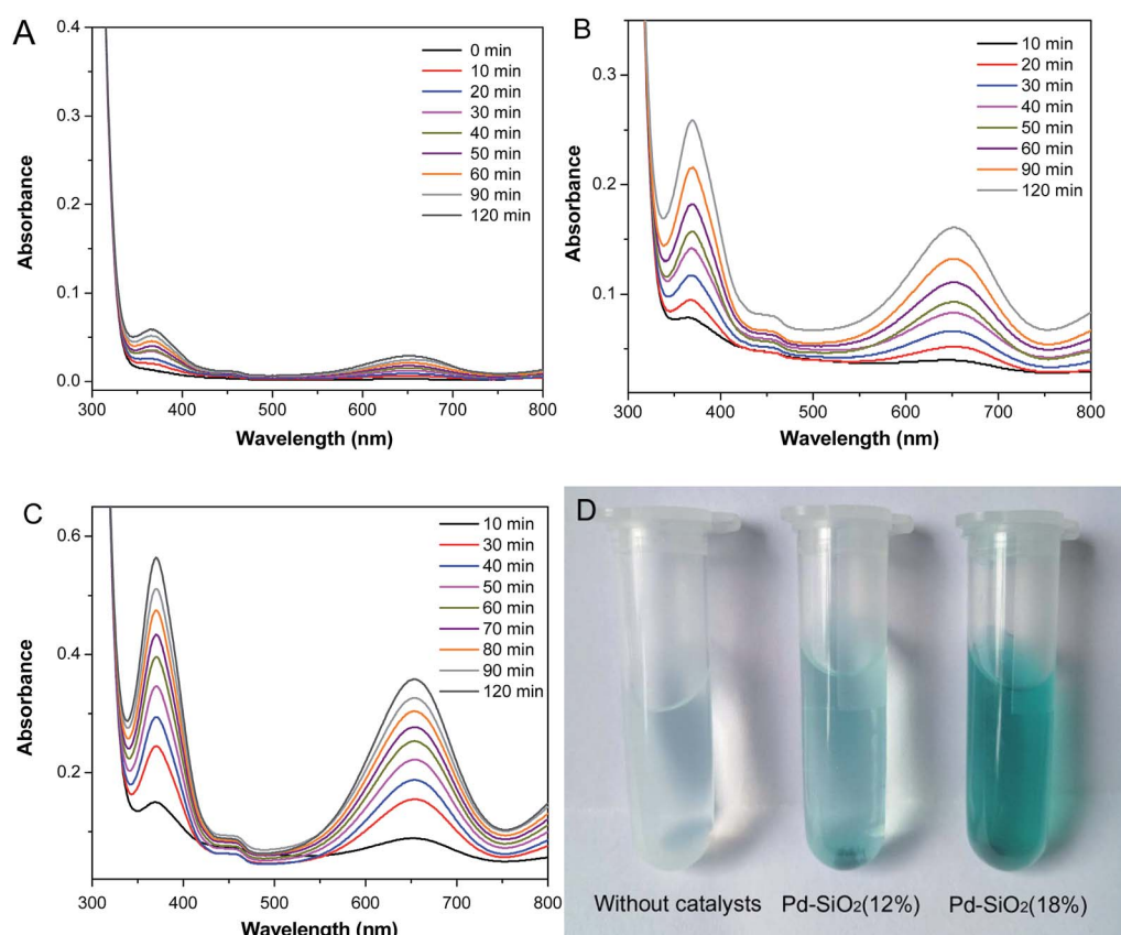
Fig. 6 Successive UV-vis absorption spectra of oxidation reaction of TMB by H 2 O 2 (A) without catalyst, and catalyzed by adding (B) Pd-SiO 2 (12%) and (C) Pd-SiO 2 (18%). (D) Corresponding digital photos of the samples.
