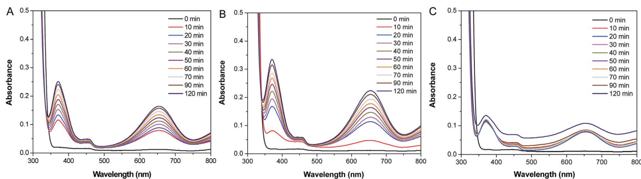
Fig. 7 Successive UV-vis absorption spectra of oxidation reaction of TMB by \text{H}_2\text{O}_2 catalyzed by adding (A) PS/ \text{C}_{16}\text{mimCl} /Pd(12%), (B) PS/ \text{C}_{16}\text{mimCl} /Pd(18%), and (C) PS/ \text{C}_{16}\text{mimCl} /Pd(24%) beads.
