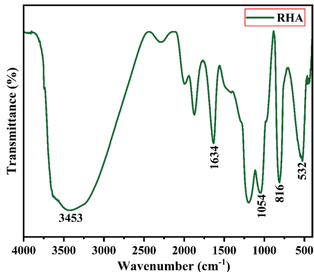
Fig. 3 FTIR spectra of Rice Husk Ash (RHA).
