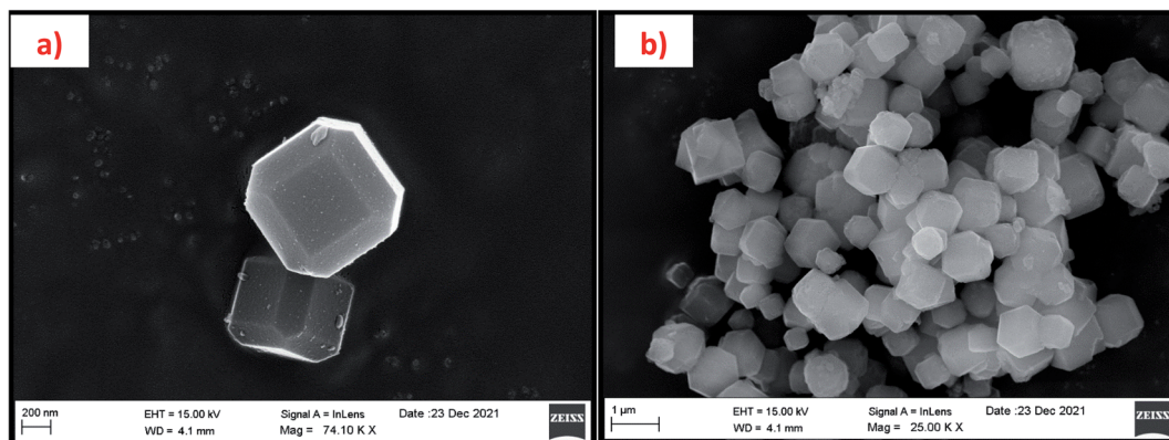
Fig. 13 (a and b) FESEM micrographs of zeolite RA synthesized from RHA at two magnifications.
