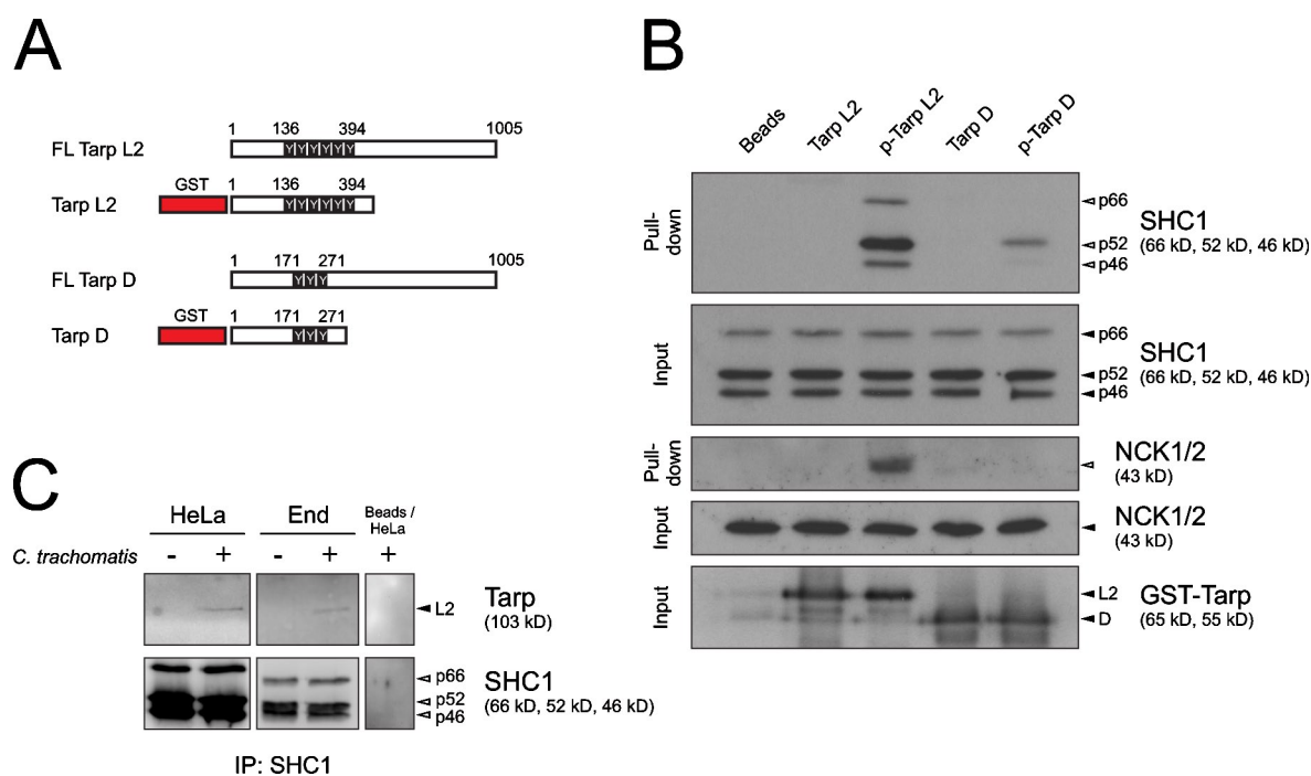
Figure 3. SHC1 is an interaction partner of Tarp D and L2. (A) Graphical representation of Tarp D and L2 and the respective GST-Tarp fusion proteins including all phospho-sites. Truncated versions of Tarp were used to avoid the actin-nucleating activity of the C terminus (Jewett et al., 2006) and any unknown binding regions. (B) Western blot showing pull-down of SHC1 and NCK2 from HeLa cell lysate using bead-coupled phospho-GST-Tarp. The fusion protein was phosphorylated in vitro with recombinant human SRC. Input shows Tarp loading (bead coupled, black arrowheads) and SHC1 and NCK2 loading in HeLa cell lysate (black arrowheads). Pulled-down SHC1 and NCK2 are indicated by open arrowheads. SHC1 was only pulled down in lanes where Tarp was phosphorylated (indicated as p-Tarp). NCK2 was only pulled down with p-Tarp L2. As a control, beads were phosphorylated in the absence of GST-Tarp and did not pull down SHC1. (C) Western blot showing coimmunoprecipitation of SHC1 (white arrowheads) and Tarp (black arrowhead) after infection of HeLa or End1/E6E7 cells ( C. trachomatis L2, MOI 500) for 60 min.
