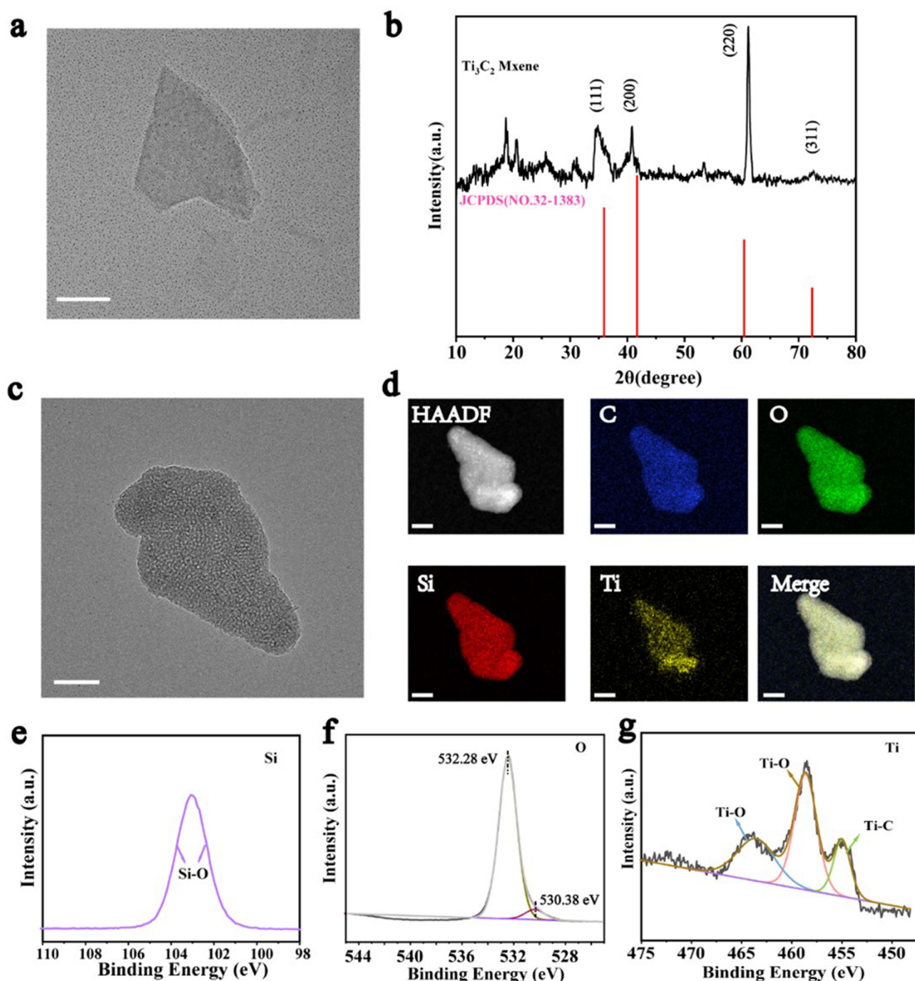
Figure 1 Synthesis and characterization of Ti_3C_2@MSNs composite nanosheets. (a) TEM image of Ti_3C_2 . Scale bar:100 nm (b) XRD pattern of Ti_3C_2 . (c) TEM image of Ti_3C_2@MSNs . (d) The corresponding elemental mappings of C, O, Si and Ti. Scale bar: 50 nm. (e) X-ray photoelectron spectroscopy (XPS) of Ti_3C_2@MSNs . (f) High-resolution O 1s and (g) Ti 2p spectra of Ti_3C_2@MSNs .
