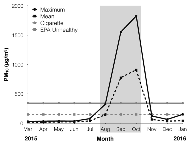
Figure 2. Maximum (solid black) and mean (dashed black) monthly PM 10 values observed in Palangkaraya across the study period. PM 10 after lighting a cigarette (solid grey) 38 and the EPA unhealthy limit (dashed grey) for reference. Light grey rectangle indicates the smoke period.
