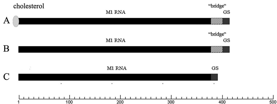
Figure 3 Schematic structure of the DNA sequences encoding M1GS ribozymes used in this study. (A) M1GS ribozyme with its guide sequence (GS) directly linked to the 3' terminus of M1 RNA. (B) M1GS ribozyme containing a bridge sequence, which is of 88 nt-length and links a GS to the 3' terminus of M1 RNA. (C) Cholesterol-modified M1GS ribozyme containing a cholesterol molecule to the 5' terminus of M1 RNA, with a bridge sequence between GS and M1 RNA.
