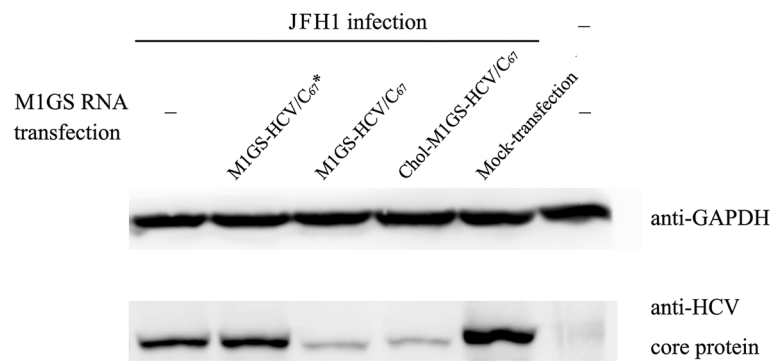
Figure 7 Levels of HCV core protein as determined by Western blot analysis. Cells were transfected with ribozymes or mock-transfected and further infected with JFH1 (MOI = 5; lanes 1–5) for 48 h. Protein samples were separated on 9% polyacrylamide gels, transferred to membranes, and analyzed with anti-HCV core protein and human GAPDH monoclonal antibodies.
