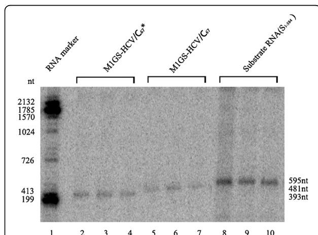
Figure 4 Determination of M1GS ribozyme transcribed in vitro by T7 RNA polymerase. The 32 P-labeled M1GS RNAs and 32 P-labeled substrate RNA (S 1-584 ) transcribed in vitro were separated on 15% polyacrylamide gels containing 8 M urea.
