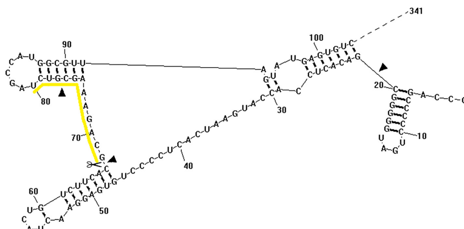
Figure 2 Secondary structure of a portion of HCV 5' UTR predicted by the RNA Structure software. The three sites indicated by triangular arrows were potential cleavage sites of M1GS ribozyme. The site indicated by scissors was an optimal cleavage site, with the sequence marked by a yellow line capable of forming a long single-strand structure and facilitating complementary binding with the GS sequence of M1GS ribozyme.
