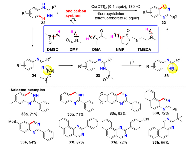
Scheme 10 Cu-catalyzed [5 + 1] annulation reactions of amidines with various one carbon synthons.
