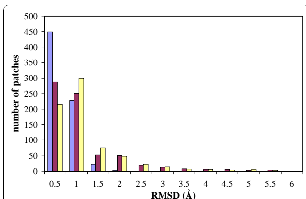
Figure 3 Quality of our rotamer library. We study the extent to which our set of rotamers can approximate the bound side-chains for our data set of 700 patches. For each patch we graft the bound side-chains onto the unbound backbone ( bound_UBB conformation) and make an alternate graft of the closest rotamers in our rotamer library ( rotamer_UBB conformation). The all-atom RMSDs between these grafts provide evidence that our rotamer library is extensive enough to produce a side-chain configuration near the bound. In all but 24 of the 700 patches this RMSD (blue, left bar) is within 1 Å. When we account for the changes in the backbone conformation between the bound and unbound conformations of the patch however, results are not as good. The maroon (center) and yellow (right) bars show the all-atom RMSD between the bound conformation of the patch and the bound_UBB and rotamer_UBB conformations, respectively. In 185 of the 700 patches, the rotamer_UBB conformation is more than 1 Å away from the bound conformation of the patch.
