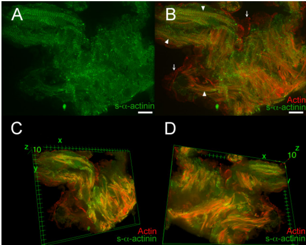
Figure 7. s- \alpha -actinin and actin organization in trabecular cardiomyocytes at embryonic day 12.5. The LifeAct-RFP rubry transgenic mouse line was used to visualize filamentous actin 19 , while the mouse monoclonal clone EA53 antibody against s- \alpha -actinin was used to label Z-discs and intercalated discs. Embryos were PFA-fixed. 0.2 \mu m optical slices were collected as a z stack. (A) Flattened z stack shows that s- \alpha -actinin staining was more diffuse in PFA-fixed tissue than in snap-frozen and acetone fixed sections ( Figures 2-5 ). (B) Flattened z stack shows both filamentous actin and s- \alpha -actinin. Filamentous actin fluorescence localized between Z-discs within myofibrils (arrowheads). Filamentous actin fluorescence was also seen in endocardial cells that line the trabecular myocytes (arrows). (C) Three-dimensional view of the trabecular cardiomyocytes, as viewed from the top of the stack. (D) Three-dimensional view of the trabecular cardiomyocytes, as viewed from the bottom of the stack. Intensity histogram display range 470-900 (out of possible 0-65535) for both the 488 nm laser channel and for the 561 nm laser channel in A and B; display range 460-800 for both channels in C and D. Scale bar 10 \mu m. Please click here to view a larger version of this figure.
