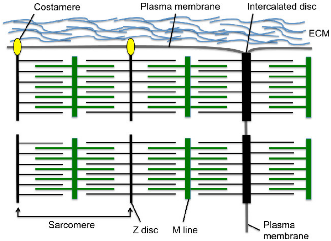
Figure 1. Cardiomyocyte sarcomeres, intercalated discs, and costameres. The Z-disc anchors actin filaments, while the M line anchors myosin fibers, which overlap the actin filaments. The sarcomere comprises one Z-disc – M line – Z-disc unit. Multiple sarcomeres in series create a myofibril. The lateral end of the myofibril inserts into the transverse border of the cardiomyocyte at a specialized cell-cell junctional structure called the intercalated disc. Peripheral myofibrils connect to the longitudinal cardiomyocyte plasma membrane via costameres, which form focal adhesions with the extracellular matrix between cardiomyocytes. Please click here to view a larger version of this figure.
