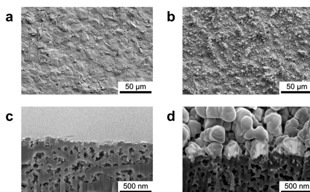
Fig. 3 FIB/FE-SEM images of the Au-NiO x -modified SPCE compared to a bare SPCE. (a) and (b) Surface morphology images of the bare and Au-NiO x -modified SPCEs, respectively. (c) and (d) Cross-sectional images of the bare and Au-NiO x -modified SPCEs, respectively.
