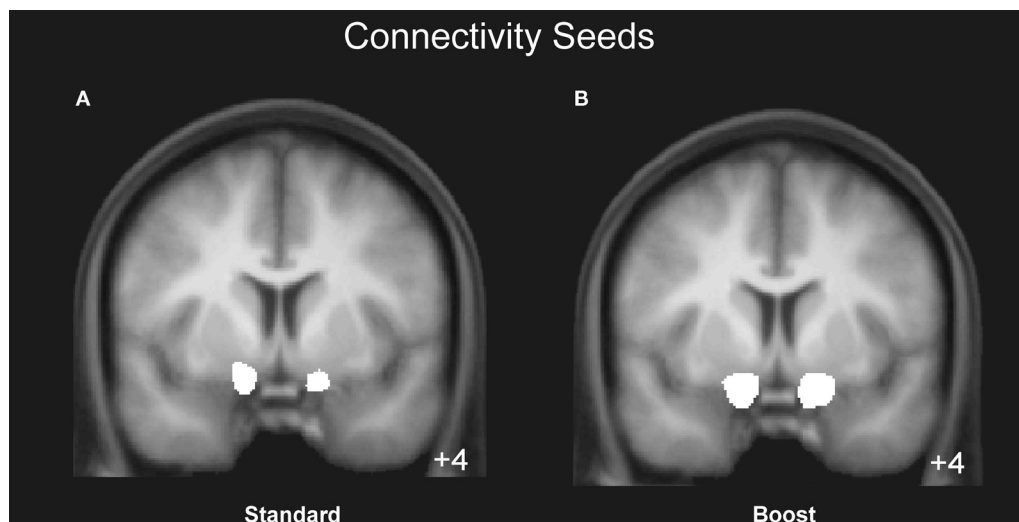
FIGURE 3 | Mean region of interest for the boost and standard condition.
