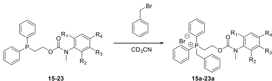
Scheme 7. Alkylation of Self-Immolative Systems 15–23 Using BnBr as an Alkylating Agent in CD 3 CN
