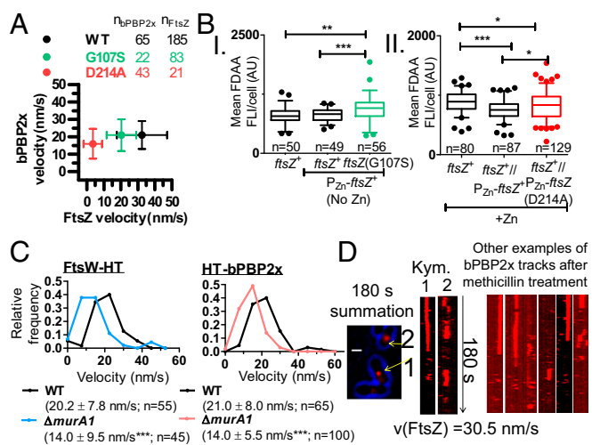
Fig. 8. S. pneumoniae bBP2x and FtsW movement depend on PG synthesis and are not correlated with FtsZ treadmilling or FtsZ(GTPase) activity. Strains were grown in C+Y, pH 6.9 at 37 °C in 5% CO 2 to OD 620 = 0.1–0.2, at which point cells were labeled with FDAA, washed, and fixed. Alternatively, cells were labeled with 120 pM HT-JF549 ligand, washed, and SM-TIRFm performed (at one frame per second) to track dynamics of HT-bBP2x or FtsW-HT. (A) Mean HT-bBP2x velocity is not correlated with FtsZ-sfGFP treadmilling velocity. Average velocities ± SDs from two or three independent biological replicates are shown for strains: IU9985 ( ftsZ-sfgfp ), IU13910 ( ht-pbp2x ), IU14375 [ ftsZ(G107S) P Zn -ftsZ-sfgfp ], IU14508 [ ftsZ(G107S) ht-pbp2x ], IU15181 [ P Zn -ftsZ(D214A) ftsZ-sfgfp ], and IU15041 [ P Zn -ftsZ(D214A) ht-pbp2x ] (SI Appendix, Experimental Procedures and Table S1 and Movies S5 and S18–S20). (B) Box-and-whisker plots (whiskers, 5th and 95th percentile) of different FtsZ(GTPase) mutants showing that mean FDAA labeling of PG per cell is not reduced in FtsZ(GTPase) merodiploid mutants (middle compared with right strains). P values were obtained by one-way ANOVA analysis (GraphPad Prism, nonparametric Kruskal–Wallis test, where * P < 0.05; ** P < 0.01; *** P < 0.001). Values are from two independent biological replicates (SI Appendix, Experimental Procedures). (C) HT-bBP2x and FtsW-HT velocity is reduced in the absence of MurA1. Velocities were determined by SM-TIRFm in strains IU13910 ( ht-pbp2x ), IU15039 ( \Delta murA1 ht-pbp2x ), IU15096 ( ftsW-ht ), and IU15173 ( \Delta murA1 ftsW-ht ) as described in Fig. 7. Shown is the average velocity ± SD of n tracks. P values were obtained by one-way unpaired, two-tailed t tests (GraphPad Prism), where *** P < 0.001. (D) HT-bBP2x movement is inhibited when cells are treated with methicillin. A final methicillin concentration of 0.3 μg/mL was added on top of an agarose pad, after which IU13910 ( ht-pbp2x ) cells were added as described in SI Appendix, Experimental Procedures. Cells were visualized by SM-TIRFm after 45–75 m of treatment with methicillin at 37 °C (Movie S22). A summation is shown of movie frames over 180 s with arrows pointing at septa where molecules of bBP2x no longer move circumferentially, as indicated by the kymographs ( n = 57). (Scale bar, 1.0 μm.) Numbers correspond to the arrows in the summation. The experiment was performed independently twice with similar results. The velocity of FtsZ-sfGFP remained unchanged, consistent with FtsZ treadmilling, independent of PG synthesis ( n = 84) (SI Appendix, Fig. S27 and Movie S21).
