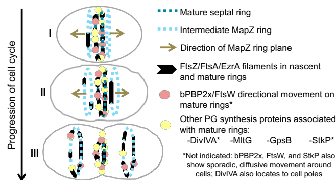
Fig. 9. Summary diagram of the movement dynamics of FtsZ, FtsA, EzrA, bBP2x, FtsW, and regulators of PG synthesis in S. pneumoniae cells. The division cycle is simplified to three stages. In early divisional cells (I), the equator becomes the septum of dividing cells, and most divisome proteins locate to the mature septum, with the exception of StkP and bBP2x, which also exhibit sporadic, diffusive movement throughout cells. bBP2x and FtsW molecules attach to the mature septal ring and move in one direction or the other for as long as 30 s. After the start of peripheral PG synthesis, MapZ bifurcates into rings on both sides of the mature septal ring, and the MapZ rings start to move outward toward the positions of the equators in the daughter cells (I–II). Concurrently, nascent filaments/bundles consisting of FtsZ and its associated proteins FtsA and EzrA are detected in MapZ rings, suggesting that MapZ rings continuously guide a fraction of FtsZ/FtsA/EzrA to new equatorial rings, where FtsZ may nucleate the transport of remaining FtsZ from the mature septal ring later in division. Treadmilling velocity and dynamics of FtsZ and EzrA are the same in mature septal, nascent, and equatorial rings, whereas FtsA may move faster than FtsZ in nascent rings. FtsZ/FtsA/EzrA filaments/bundles accumulate as nascent MapZ rings move away from the mature septal ring and become early equatorial rings in daughter cells. Directional movement in or association with nascent rings was not detected for PG synthesis proteins bBP2x, FtsW, DivIVA, MltG, StkP, and GpsB, and these PG synthesis proteins remain at constricting septa until migrating to new equatorial rings late in cell division, where bBP2x and FtsW form a complex and move circumferentially in either direction (III). The movement of bBP2x:FtsW complexes in septal PG synthesis depends on and reflects new PG synthesis and is not correlated with the treadmilling of FtsZ filaments/bundles. See Discussion for additional details.
