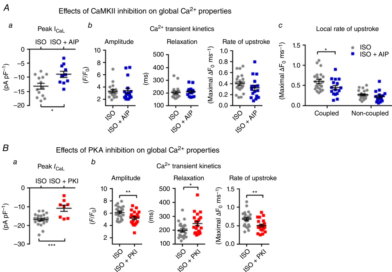
Figure 10. Global Ca^{2+} handling is increased during \beta -adrenergic stimulation via global PKA effects and local CaMKII effects
