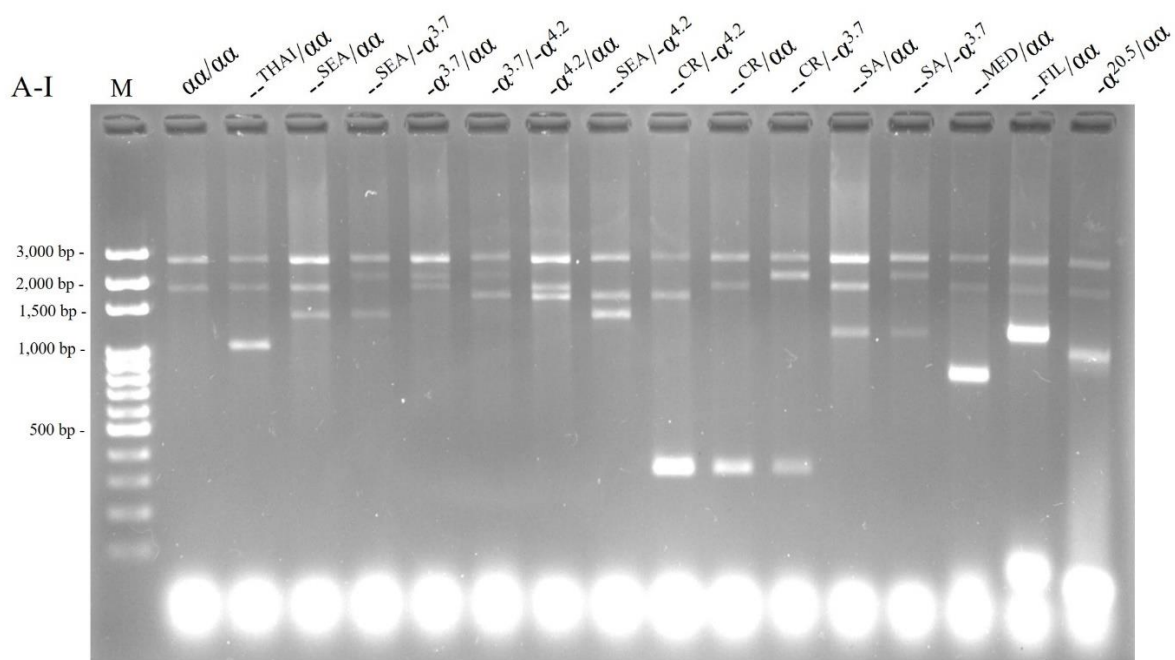
Supplementary Figure 1 Original agarose gel electrophoresis results of 21 \alpha -thalassemia genotypes (AI-III).
