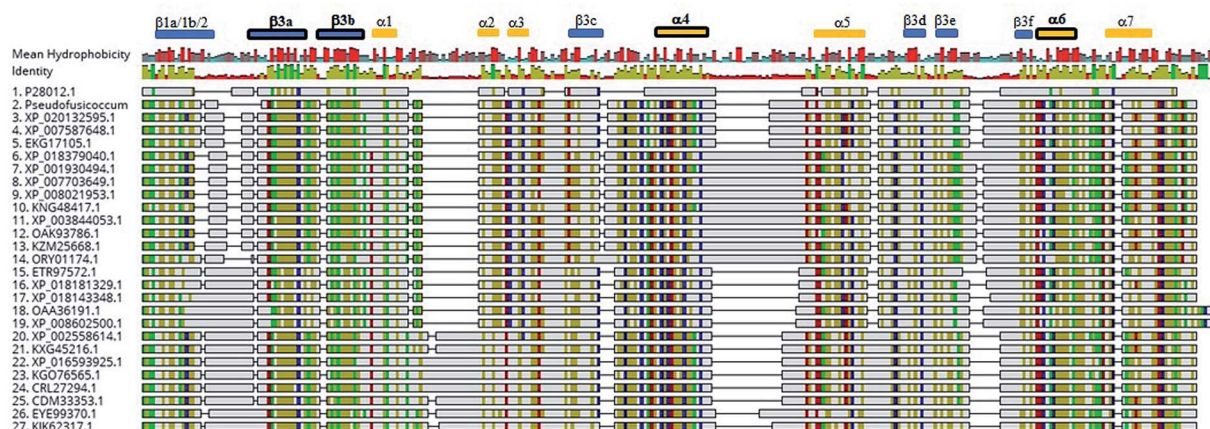
Fig. 5 Alignment of fungi CHI-like and referential plant CHI amino acid sequences. Legend: 1 – Medicago sativa , P28012, 2 – Pseudofusicoccum stromaticum ; 3 – Diplodia corticola , XP_020132595.1; 4 – Neofusicoccum parvum UCRNP2, XP_007587648.1; 5 – Macrophomina phaseolina MS6, EKG17105.1; 6 – Alternaria alternata , XP_018379040.1; 7 – Pyrenophora tritici-repentis Pt-1C-BFP XP_001930494.1; 8 – Bipolaris sorokiniana ND90Pr, XP_007703649.1; 9 – Setosphaeria turcica Et28A, XP_008021953.1; 10 – Stemphylium lycopersici , KNG48417.1; 11 – Leptosphaeria maculans JN3, XP_003844053.1; 12 – Stagonospora sp. SRC1sM3a, OAK93786.1; 13 – Ascochyta rabiei , KZM25668.1; 14 – Clohesyomyces aquaticus ORY01174.1; 15 – Trichoderma reesei RUT C-30, ETR97572.1; 16 – Purpureocillium lilacinum , XP_018181329.1; 17 – Pochonia chlamydsposoria 170, XP_018143348.1; 18 – Cordyceps brongniartii RCEF 3172, OAA36191.1; 19 – Beauveria bassiana ARSEF 2860, XP_008602500.1; 20 – Penicillium chrysogenum XP_002558614.1; 21 – Penicillium griseofulvum , KXG45216.1; 22 – Penicillium expansum , XP_016593925.1; 23 – Penicillium italicum , KGO76565.1; 24 – Penicillium camemberti , CRL27294.1; 25 – Penicillium roqueforti FM164, CDM33353.1; 26 – Aspergillus ruber CBS 135680, EYE99370.1; 27 – Aspergillus parasiticus SU-1, KJK62317.1. Secondary structure of CHI from Medicago sativa (alfalfa; P28012) is shown on top of the figure, with \alpha -helices and \beta -strands shown in gold and blue rectangles respectively. \alpha -helices and \beta -strands forming the substrate-binding clef are highlighted in bold.
