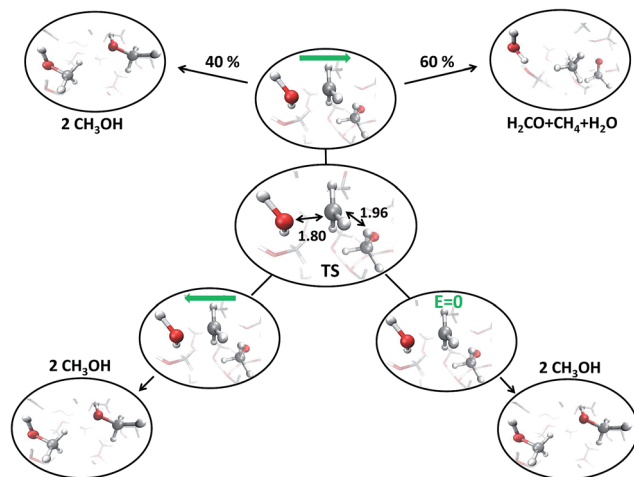
Fig. 7 Transition state (TS) (center) for a field strength of 0.30 \text{ V \AA}^{-1} , as confirmed by the committor analysis shown in the upper part; some relevant distances (in Å), such as the CO and the CH lengths are highlighted. Comparing them with the zero-field case: in the presence of the field the reaction is “anticipated”, with the TS more resembling the reactant configuration. By launching 40 independent AIMD simulations from the TS, 40% and 60% of them fall in the reactant and product basin, respectively. From the center to the lower part, the same analysis is shown by applying in one case a reversed electric field direction, whereas in the other case the zero-field has been also tested for a one-to-one comparison with the zero-field case of Fig. 6. In both cases, the reaction is always inhibited ( i.e. , 100% of the trajectories fall into the reactant state).
